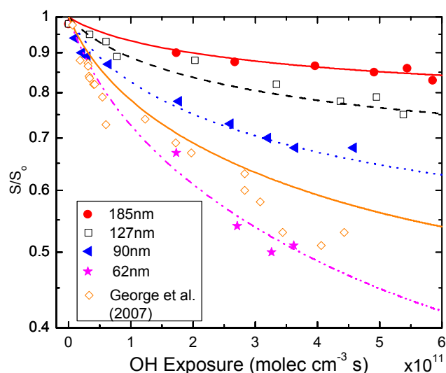
Fig. 4. Palmitic acid remaining for pure particles of four different sizes, 185 nm (●), 127 nm (□), 90 nm (◄), and 62 nm (★) versus OH exposure. Data shown as diamonds are those of George, et al. (2007). Symbols represent experimental data and the lines represent model predictions for the respective sizes.
