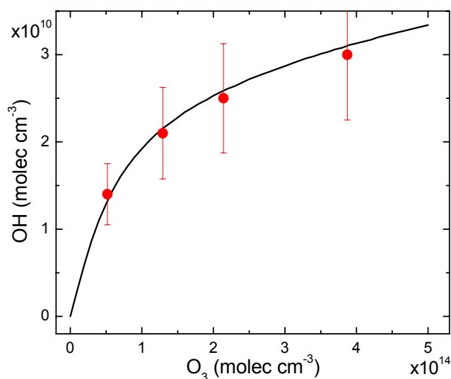
Fig. 2. OH predicted by the photochemical box model (line) compared to that calculated from SO 2 loss experiments (circles). Error bars represent 25% uncertainty in OH calibration data.
