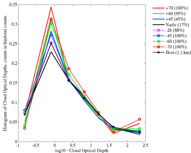
Figure A2. Same as Figure A1 but for the tropical western Pacific, July 2001.
