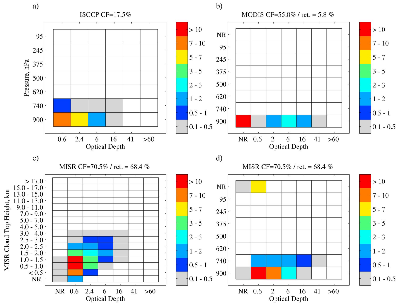
Figure 4. Joint histograms of cloud top height and optical depth for scene shown in Figure 3. Results for (a) ISCCP, (b) MODIS, (c) MISR, and (d) MISR mapped onto ISCCP/MODIS vertical pressure grid.
