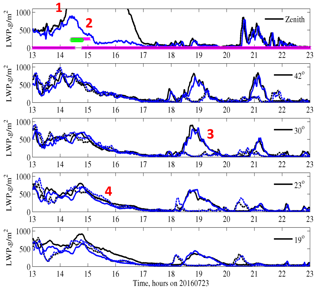
Figure 3 – LWP retrieval for lightly precipitation case (7/23/2016).
