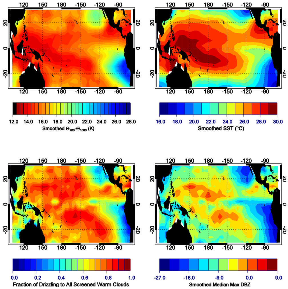
Fig. 3. (a) Smoothed 700mb-1000mb \Delta\Theta (K), (b) smoothed SST( ^{\circ} C), (c) fraction of drizzling to screened warm clouds, (d) median max dBZ.
