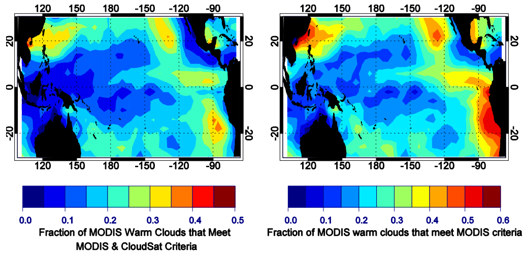
Fig. 1. (a) Fraction of MODIS warm clouds that CloudSat can sense that have \tau > 3 and a cloud fraction of one for all individual MODIS pixels, (b) Fraction of MODIS warm clouds that have \tau > 3 and a cloud fraction of one for all individual MODIS pixels. See text for details.
