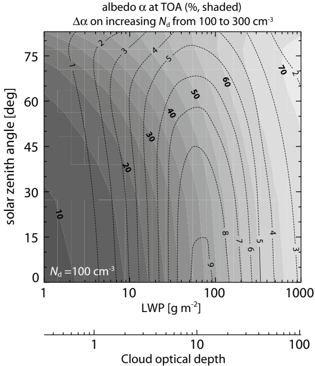
FIG. 20. Broadband solar albedo (at the top of the atmosphere) for an adiabatic plane-parallel liquid water cloud with a cloud droplet concentration of N_d=100\text{ cm}^{-3} as a function of the cloud liquid water path (LWP) and the solar zenith angle (shaded contours). Solid lines show the increase in albedo (upon increasing N_d from 100 to 300\text{ cm}^{-3} ). Calculations use the Fu–Liou two-stream radiative transfer code. The tropical dry thermodynamic profile used is described in Caldwell et al. (2005).
