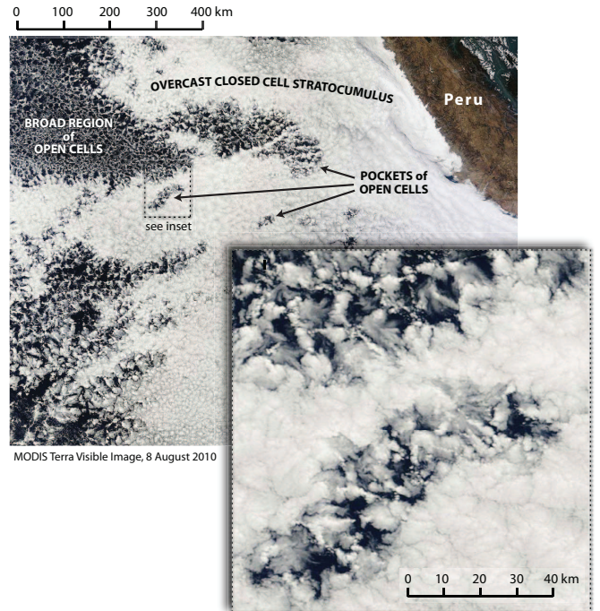
FIG. 27. Visible imagery from MODIS on the NASA Terra satellite showing Pockets of Open Cells (POCs) embedded in overcast closed cell marine stratocumulus over the tropical southeastern Pacific Ocean. The inset shows an enlarged region detailing the cellular structure within a POC.
