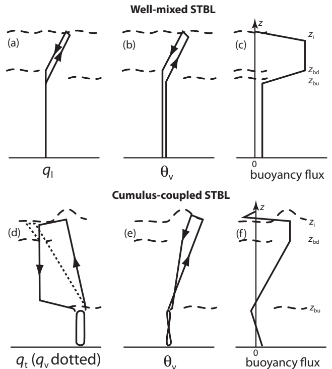
FIG. 22. “Schubert” diagrams indicating air typical air parcel circuits (a,b,d,e) and buoyancy flux profiles (c,f) through STBLs that are well-mixed (a–c) and cumulus-coupled (d–f). For the well-mixed case, (a) liquid water mixing ratio q_l and (b) virtual potential temperature \theta_v circuits are shown, while the cumulus-coupled case shows (d) total water q_t and vapor q_v mixing ratios, and (e) \theta_v are shown. Wavy dashed lines indicate heights of updraft and downdraft condensation levels z_{bu} and z_{bd} respectively, and inversion height z_i . Reproduced from Bretherton (1997) with the author’s permission.
