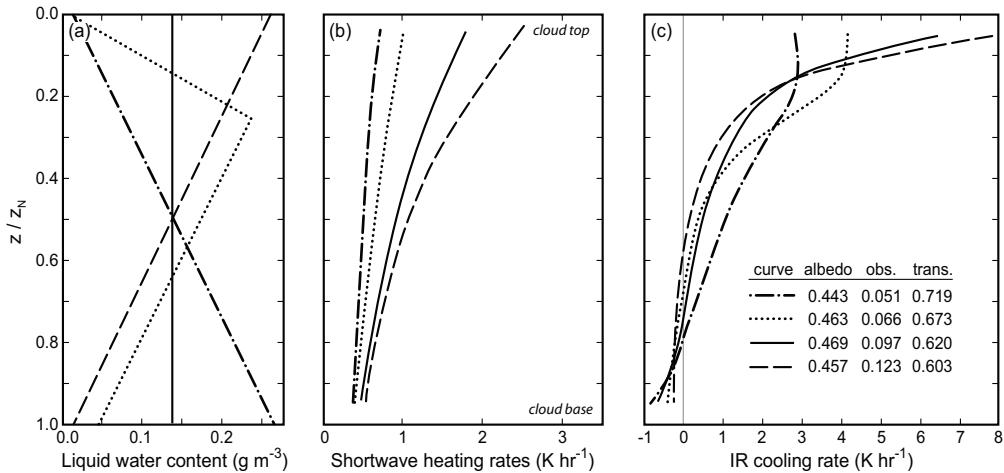
FIG. 19. Comparison of shortwave heating rates (center panel) and longwave cooling rates (right panel) in a stratocumulus-like idealized cloud layer (320 m thick, LWP=44 g m -2 ) for different vertical profiles of liquid water content (left panel). From Stephens (1978a). (c) American Meteorological Society. Reprinted with permission. The meteorological conditions are described in Stephens et al. (1978), with a downwelling solar irradiance at the top of the cloud of 880 W m -2 typical for the subtropics around noon.
