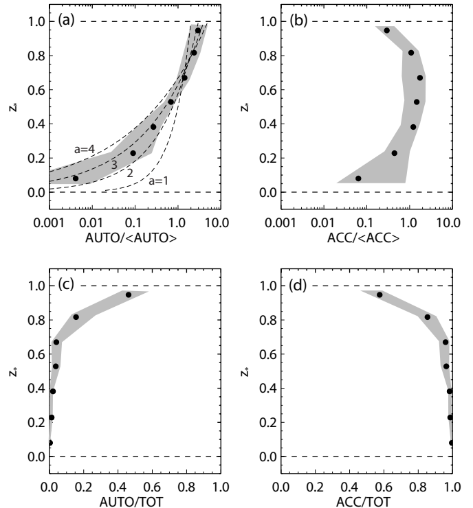
FIG. 24. Composite profiles from 12 cases of weakly to moderately drizzling stratocumulus of (a) autoconversion and (b) accretion rate normalized with the case mean in each case. The normalized height z_* is 0 at cloud base and 1 at cloud top. The process rates were derived by applying the SCE to observed drop size distributions. The lower panels show the fraction of total drizzle liquid water content production rate (autoconversion+accretion) contributed by (c) autoconversion and (d) accretion. In all plots solid circles are median values for each height bin; gray area encompass 25th and 75th percentiles. The dashed curves in (a) show the autoconversion rate expected for a cloud with a linear increase in cloud liquid water content with height and where autoconversion depends upon liquid water content to the power b , with b = 1, 2, 3, 4 . From Wood (2005b). (c) American Meteorological Society. Reprinted with permission.
