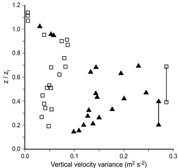
FIG. 21. Variance of the vertical wind against height normalized by the STBL depth around local noon (open squares) and for 9:30–midnight (filled triangles). Measurements were made from a tethered balloon at San Nicholas Island in unbroken Californian marine stratocumulus sheet during July 1987. The range of cloud base height for the two periods is depicted by the vertical lines. Reproduced from Hignett (1991). (c) American Meteorological Society. Reprinted with permission.
