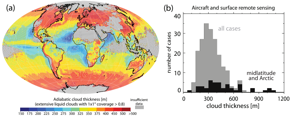
FIG. 5. (a) Annual mean cloud thickness for horizontally-extensive liquid cloud (instantaneous coverage exceeding 80% at the 1 \times 1^\circ scale). Adiabatic thickness is deduced from MODIS Terra liquid water path estimates at \sim 10:30 local time (close to the time where the cloud thickness is close to the mean daily value), and is based on the assumption that the clouds are adiabatic (Section 3a). The vertical liquid water gradient is estimated using the MODIS-derived cloud top temperature. Wood and Bretherton (2004) has additional details. (b) compilation of measurements of stratocumulus cloud thicknesses from observational case studies using aircraft and ground-based remote sensing, with all cases (gray) and midlatitude and Arctic cases (black) presented separately. Data are from the published literature and available datasets from recent stratocumulus field campaigns (Nicholls and Leighton 1986; Boers and Krummel 1998; Miles et al. 2000; Pawlowska and Brenguier 2003; Comstock et al. 2004; vanZanten et al. 2005; Wood 2005a; Lu et al. 2007; McFarquhar et al. 2007; Lu et al. 2009; Wood and coauthors 2011)
