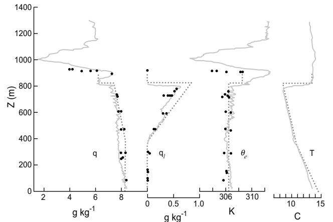
FIG. 10. Vertical profiles of water vapor q and liquid water q_l mixing ratios, equivalent potential temperature \theta_e and temperature T for a summertime shallow and quite well-mixed STBL observed over the North Sea to the east of a ridge. Means from horizontal legs are depicted by dots. The dotted lines in each case show the values expected for a well-mixed layer. Adapted from Nicholls (1984).
