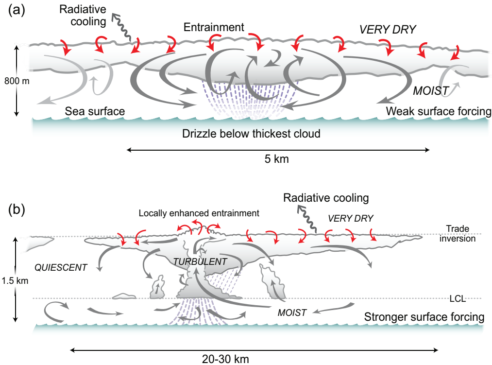
FIG. 15. Schematic showing structure of marine stratocumulus in (a) the shallow, well-mixed boundary layer; (b) deeper, cumulus-coupled boundary layers. Gray arrows indicate the primary motions on the scale of the boundary layer, while smaller red arrows indicate the small-scale entrainment mixing taking place at the inversion atop the layer. Vertical thermodynamic profiles associated with the two schematics are roughly represented by the (a) the FIRE SNI and (b) the ASTEX VALD profiles shown in Fig. 14.
