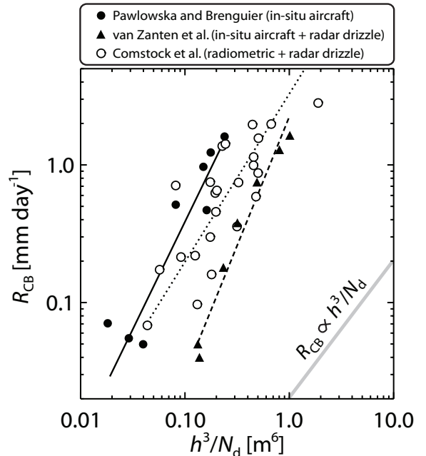
FIG. 25. Cloud base precipitation rates R_{cb} from observational case studies in subtropical marine stratocumulus, plotted against the ratio of the cube of the cloud thickness h to the cloud droplet concentration N_d . The lines represent linear least-distance regressions to the case studies for each field campaign. From Brenguier and Wood (2009).
