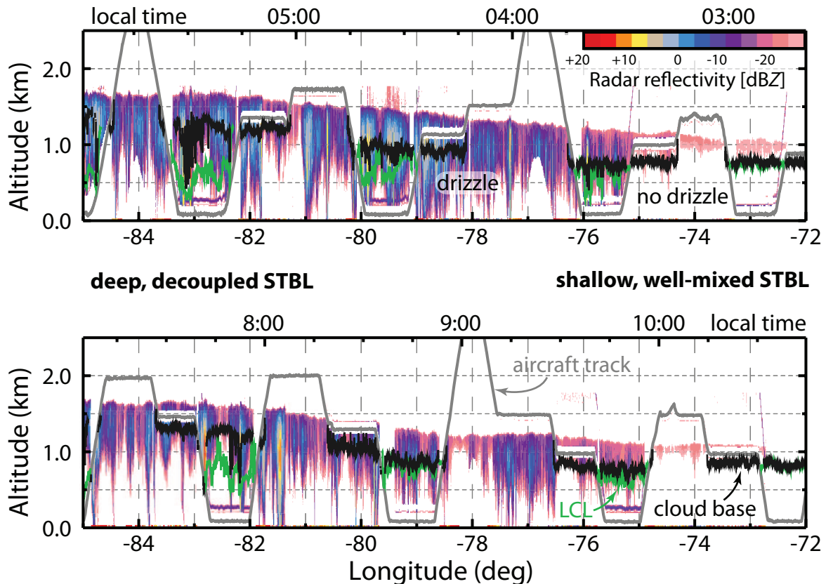
FIG. 16. Observed spatial transition from a shallow, well-mixed STBL (right) to a deeper, decoupled STBL (left). Longitude-height plot of radar reflectivity (color scale at top right) measured using an up/down pointing millimeter radar on a research aircraft flying along 20^\circ S latitude line from the coast of northern Chile ( 70^\circ W, right) to the remote southeastern Pacific Ocean ( 85^\circ W, left) on 21 October 2008 during the VOCALS Regional Experiment (Wood and coauthors 2011). The outbound (top) and return (bottom) portions of the flight are shown. The aircraft track is indicated by the gray line. During flight legs below cloud, the in-situ lifting condensation level (green) and upward-pointing lidar cloud base (black) are superimposed. During cloud legs, the black line shows the cloud base adiabatically derived from in-situ liquid water content measurements. The top axis labels show local time. Adapted from Fig. 2 of Bretherton et al. (2010a). Reproduced/modified with the author's permission.
