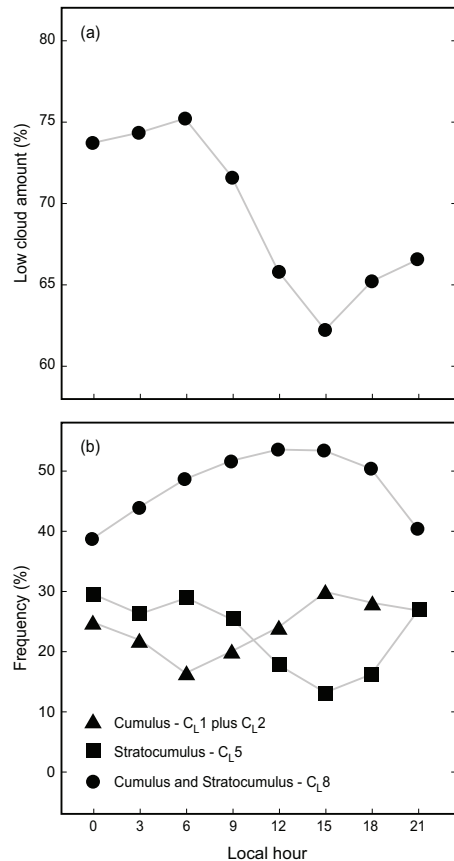
FIG. 8. Mean summertime (June–September) diurnal cycle of (a) low cloud amount; (b) frequency of occurrence of different WMO low-cloud types for cases of cold advection at 30^\circ\text{N}, 140^\circ\text{W} , a region of stratocumulus to cumulus transition. From Klein et al. (1995). (c) American Meteorological Society. Reprinted with permission.
