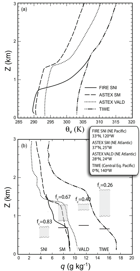
FIG. 14. Composite mean profiles of (a) virtual potential temperature \theta_v ; (b) water vapor mixing ratio from four marine field studies located in regions with distinctly different marine boundary layer characteristics: just off the Californian coast (San Nicholas Island, SNI); the subtropical/midlatitude eastern Atlantic (Santa Maria Island in the Azores, SM); the subtropical Atlantic (R/V Valdivia , VALD); the equatorial central Pacific (Tropical Instability and Waves Experiment, TIWE). See Albrecht et al. (1995b) for details of the locations. On panel (b) is indicated mean inversion base heights and cloud bases (indicated with cloud extent), lifting condensation levels (horizontal lines), and cloud cover f_c . Figure adapted from Fig. 2 and Table 2 of Albrecht et al. (1995b). Reproduced/modified by permission of American Geophysical Union.
