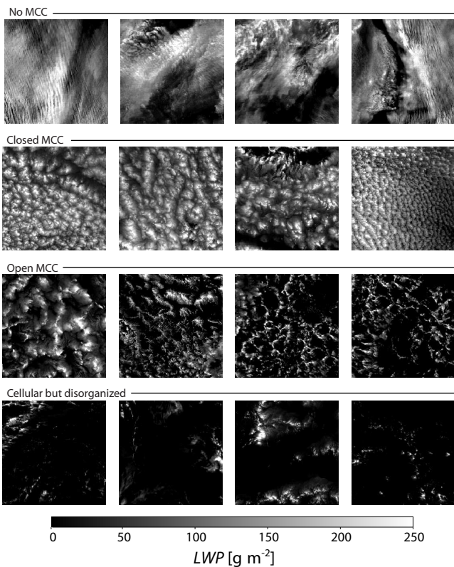
FIG. 9. Examples of different mesoscale structure types occurring in marine stratocumulus. Each image is 256 \times 256 km in size and shows liquid water path estimated using the Moderate Resolution Imaging Spectroradiometer (MODIS). Note that visible reflectance imagery would look almost identical. Reproduced from Wood and Hartmann (2006), (c) American Meteorological Society. Reprinted with permission.
