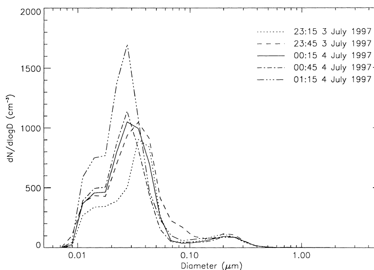
Fig. 8. The variation of the aerosol size spectra measured by the R/V Vodyanitskiy an hour either side of the release of the constant height "smart" balloons at the start of the 1st Lagrangian experiment. The aerosol was dried to a RH of 50%. All times are in GMT.
