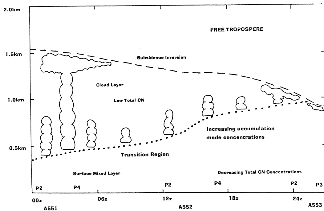
Fig. 6. A schematic diagram of the boundary layer, cloud and aerosol evolution during the 1st Lagrangian experiment.
