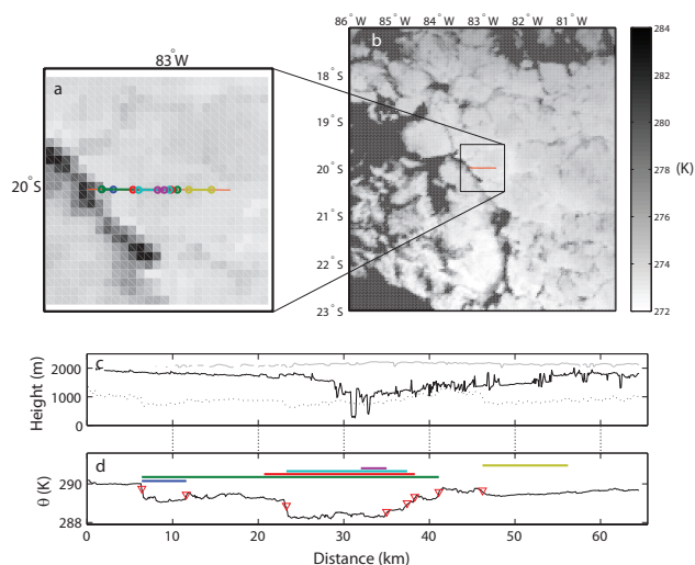
Fig. 3. The top panels show the GOES-10 satellite imagery from 11 \mu\text{m} channel in a 1^\circ (a) and 6^\circ square box (b) centered on the flight leg (orange) taken during the flight leg (23 October 2008 at 10:28 UTC). (c) Corresponds to Fig. 1a, where cloud top height (gray), cloud base height (solid black), and LCL (dotted) are shown. The \theta time series in (d) shows the location and size of cold pools detected by the algorithm described in the text. Each colored segment over the \theta time series represents an individual cold pool.
