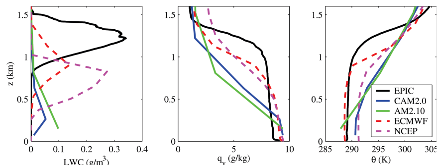
FIG. 10. Comparison of 6-day buoy-period mean cloud and thermodynamic profiles—liquid water content (LWC), water vapor ( q_v ), and potential temperature ( \theta )—from EPIC with ECMWF and NCEP–NCAR operational analyses for the same time and location, and with Oct climatological profiles for recent versions of two leading GCMs.
