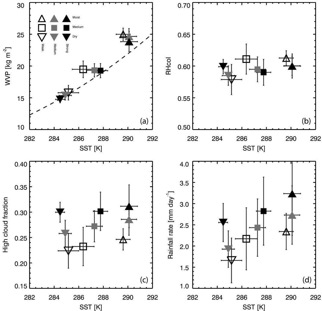
FIG. 12. Mean cyclone composite values within a 2000-km circle centered on x = 0 , y = 0 . Error bars represent the error in the mean at 95% confidence. These are obtained by calculating the weighted mean of the standard errors at each point in the composite, and then dividing by the square root of the degrees of freedom in the composite field that are determined using the spatial equivalent of the temporal autocorrelation method of Leith (1973). SST against (a) WVP [the dashed line represents the expected relationship from a water vapor feedback argument; see Curry and Webster (1999)]; (b) column relative humidity RH_{col} , (c) high cloud fraction, and (d) rain rate.
