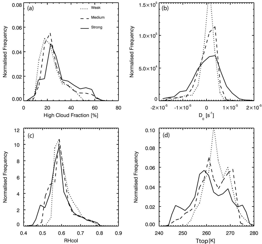
FIG. 11. Frequency distributions showing spatial variability across the 18 \langle \text{WVP} \rangle < 21 \text{ kg m}^{-2} composites of (a) high-cloud fraction, (b) horizontal surface wind divergence D_0 , (c) column-relative humidity \text{RH}_{\text{col}} , and (d) cloud-top temperature T_{\text{top}} .
