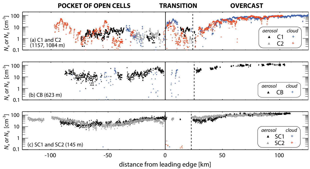
Fig. 016. Cloud droplet concentration from the CDP N_d (colored crosses, samples in cloud) or PCASP aerosol concentration N_a (black or gray triangles, clear air samples) for (a) cloud layer legs C1 and C2; (b) cloud-base level leg CB; (c) subcloud legs SC1 and SC2. The data are plotted each second as a function of the distance from the leading edge of the transition region (positive towards the overcast region). Each 1 Hz data point is classified as either cloudy or clear using the criteria described in Section 2.4. Drizzle-containing points are excluded from the analysis since the aerosol measurement is prone to shattering artifacts.
