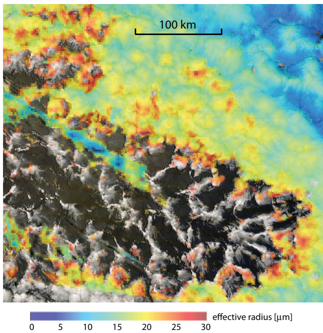
Fig. 013. MODIS-estimated cloud top effective radius r_e (colors) from the 2.1 \mu\text{m} near-IR channel, overlaid on MODIS 250 m visible imagery which is revealed where r_e retrievals are not performed because 1 km pixels used for the retrieval are determined to be partially filled, too optically thin, or are cloud edge pixels.
