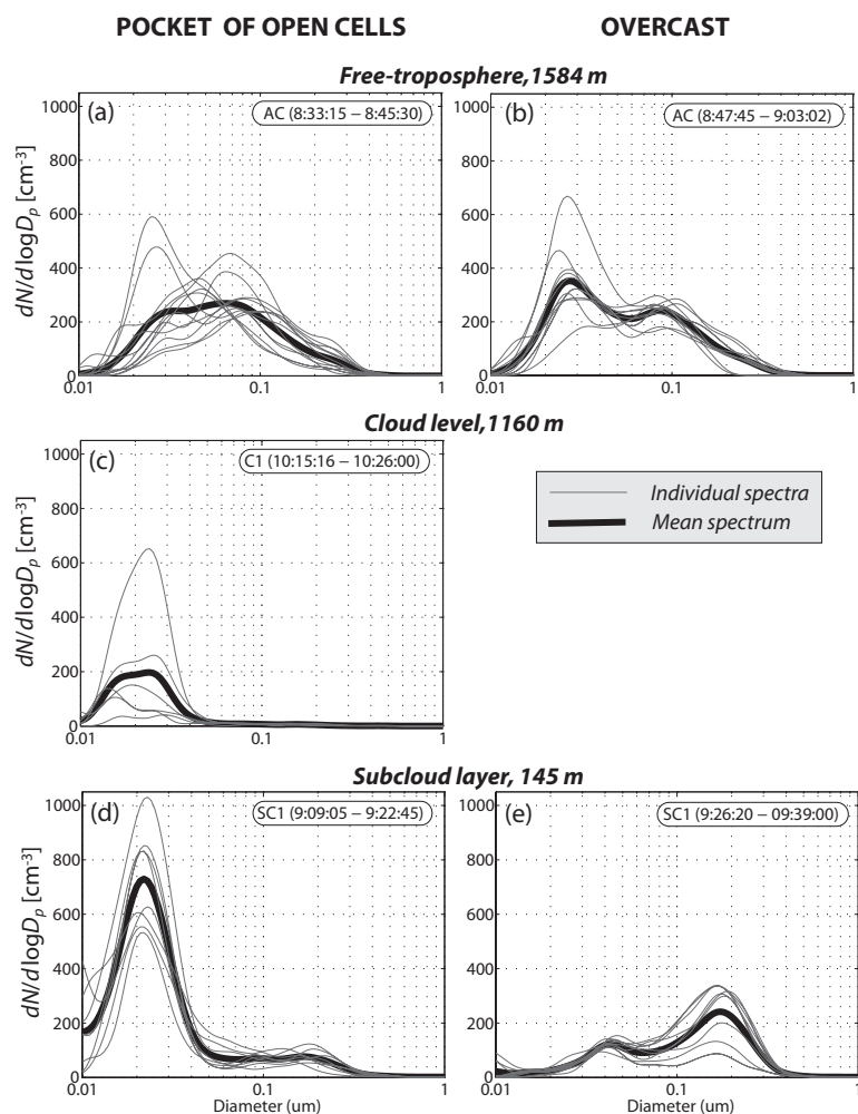
Fig. 014. Aerosol size distributions for clear-air samples measured with the University of Hawaii in-cabin sampling system, at different levels in the POC region (a,c,d for the free-troposphere, cloud level, and subcloud layer respectively) and for the overcast region (b and e for the free-troposphere and subcloud layers respectively). We show both individual spectra (typically taken over 10 s samples) and the mean spectrum for each level/region, to emphasize variability. No data are available from the cloud level in the overcast region since almost the entire leg was cloudy.
