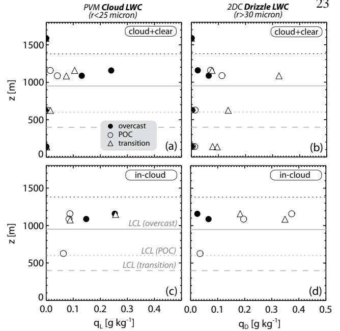
Fig. 07. Profiles of mean values of cloud (a,c) and drizzle (b,d) liquid water content from straight and levels runs (symbols) in the POC, overcast, and transition regions. The upper panels (a,b) give values averaged over both cloudy and clear portions of the legs, while the lower panels (c,d) show values averaged over cloudy samples only. Note that there is little difference between the cloud+clear and in-cloud values for the overcast region since the runs were either almost entirely in cloud or entirely out of cloud.
