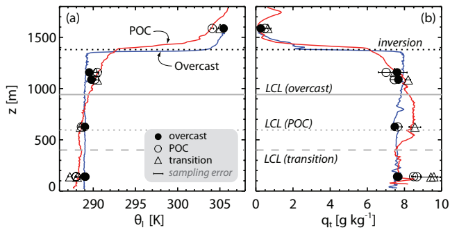
Fig. 06. Profiles of mean values of (a) liquid potential temperature and (b) total water content, from straight and levels runs (symbols) in the POC, overcast, and transition regions. Representative example profiles are also shown for the POC (red, 120 km from boundary, 1255-1305 UTC) and overcast (blue, 160 km from boundary, 1050-1056 UTC) regions. Profile locations are shown in Fig. 03.
