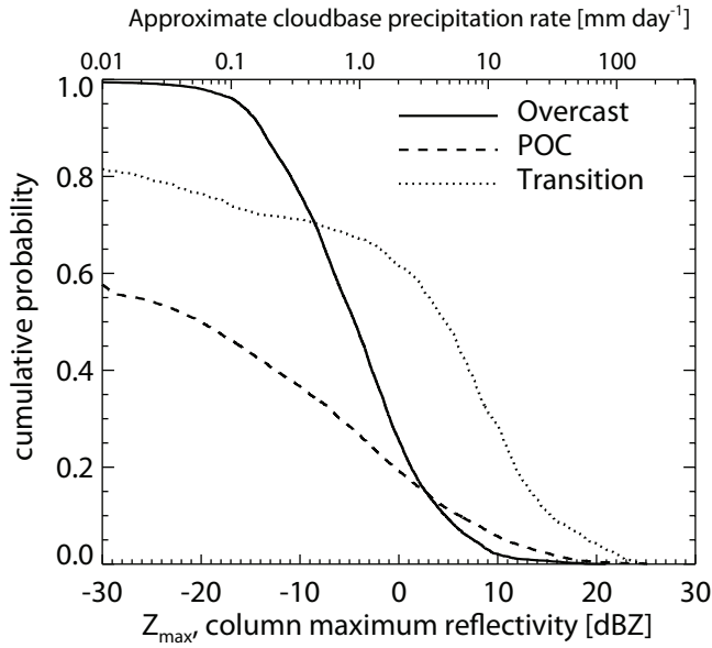
Fig. 05. Cumulative probability of column maximum radar reflectivity Z_{\text{max}} greater than the abscissal value, for the overcast (solid), POC (dashed), and transition (dotted) regions. All available WCR data from all flight legs were used to construct the plot. The top axis denotes the approximate cloudbase precipitation rate corresponding to Z_{\text{max}} constructed using the Z - R relationship discussed in Section 2.3.
