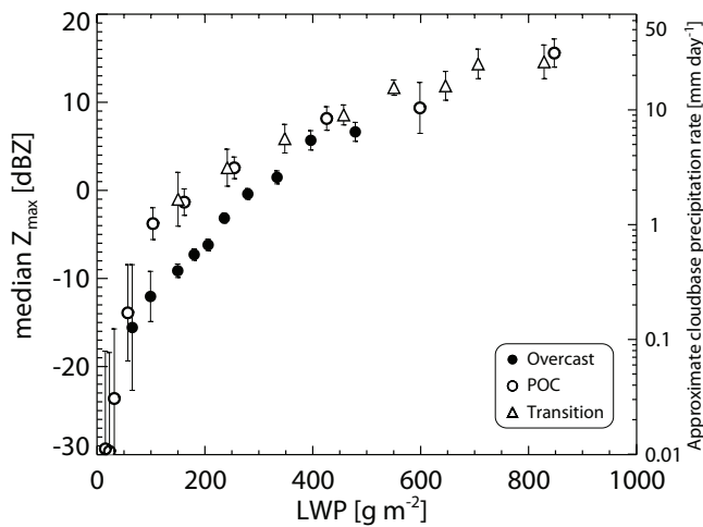
Fig. 012. Median column maximum reflectivity Z_{max} for all samples on which the WCL detected clouds above, binned as a function of LWP in the overcast (solid circles), POC (open circles), and transition (open triangle) regions. All data from the two subcloud legs SC1 and SC2 are used. The right axis denotes the approximate cloudbase precipitation rate corresponding to Z_{max} constructed using the Z - R relationship discussed in Section 2.3.
