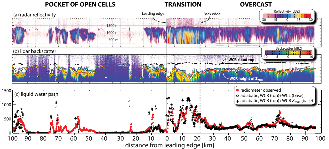
Fig. 011. Time series, from leg SC2, of (a) WCR radar reflectivity; (b) WCL lidar backscatter, with WCR cloud top (1 Hz) and the height of the maximum WCR reflectivity (smoothed with 7 second triangular filter and plotted every fifth point for clarity) overlaid; (c) liquid water path from the microwave radiometer (red circles) and estimated using two adiabatic models. Both models use the WCR observed cloud top height, but one uses the lidar-derived cloud base height where available (open circles), and the other uses the height of the maximum WCR radar reflectivity as a proxy for the cloud base height (crosses) where strong drizzle precludes accurate WCL cloud base height estimates.
