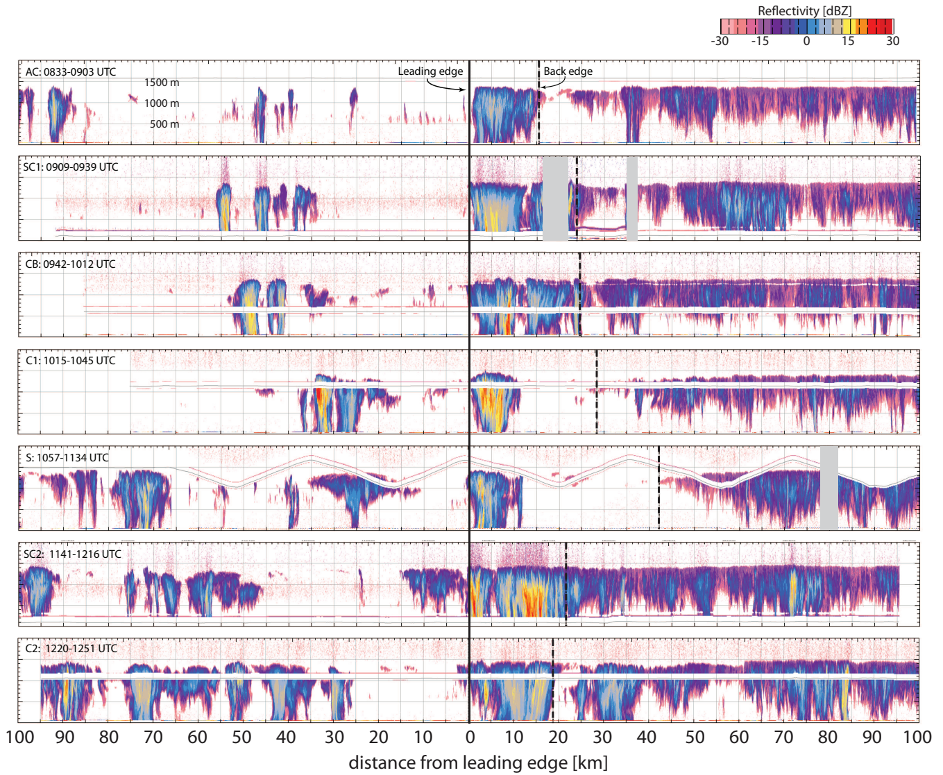
Fig. 04. Radar cross sections from the WCR for all legs in RF06. Runs are presented in time order (earliest at top). Gray regions denote periods when WCR was not functional.
