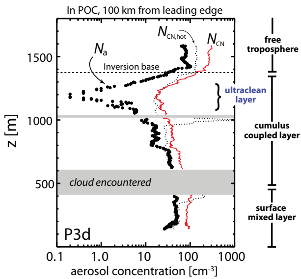
Fig. 015. Representative profile (Profile 3d) within the POC of aerosol concentration N_a measured with the PCASP (solid circles), the CN counter (red) and with the CN counter after heating to 250 C (short-dash) in the POC region approximately 100 km from the leading edge.
