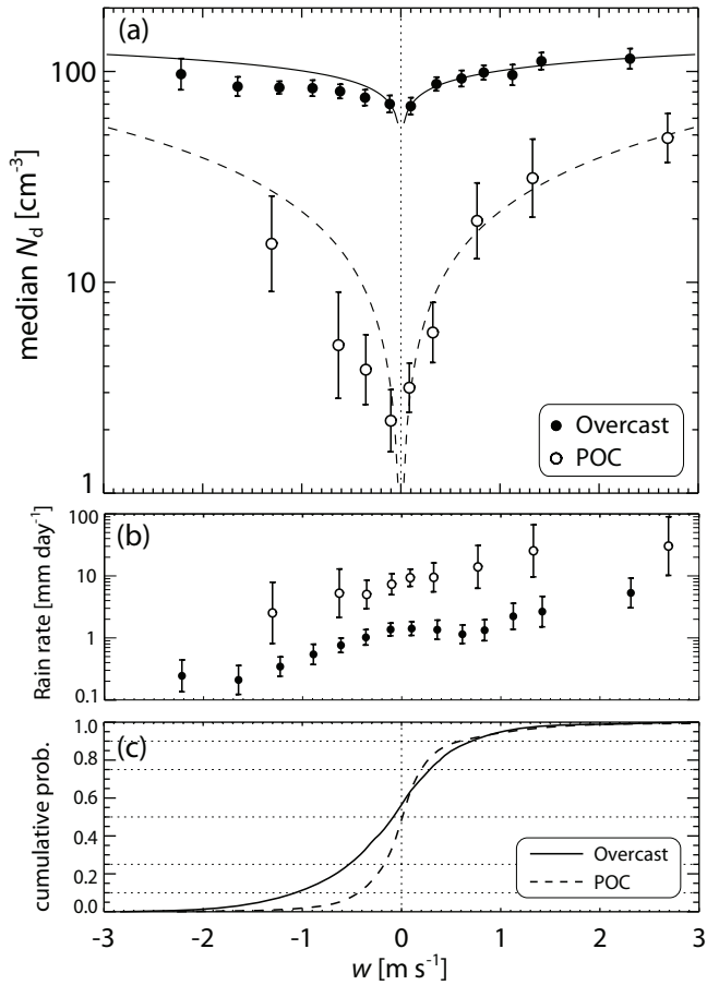
Fig. 017. (a) Median droplet concentration N_d for cloudy samples (see Section 2.4) binned as a function of the sample's vertical wind w magnitude in the overcast (solid circles) and POC (open circles) regions. Error bars show the approximate 95% confidence interval for the medians with degrees of freedom estimated using the approximately exponential decay of the autocorrelation function. Panel (b): rain rate from the 2D-C probe for cloudy samples binned as a function of w as in (a). Panel (c): cumulative distribution function of the vertical wind from the cloud data in the overcast and POC regions.
