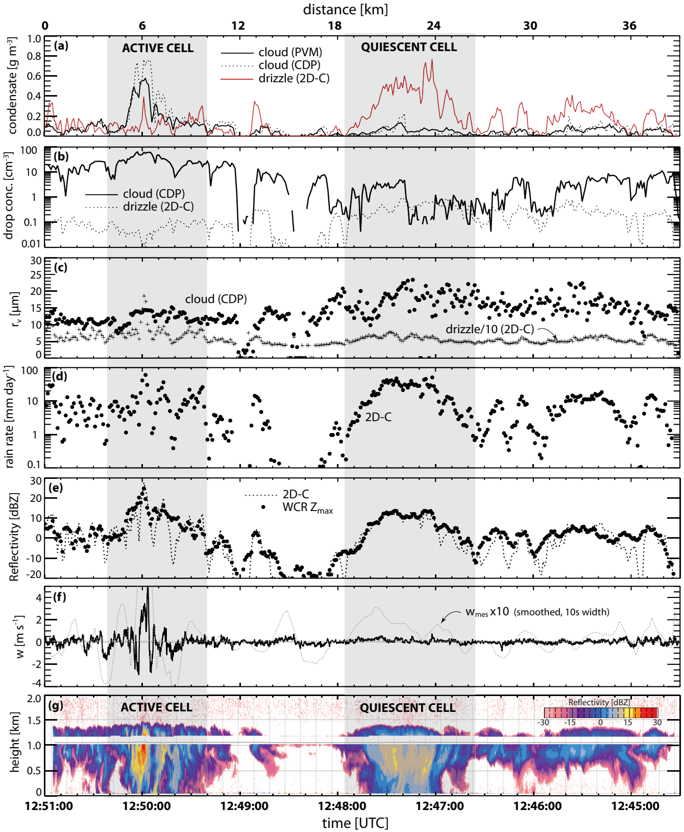
Fig. 019. Time series for 6.5 minutes ( \sim 40 km) from leg C2 at an altitude of 1084 m contrasting two cells producing strong drizzle. The panels show: (a) Condensed water content for cloud water (both from the PVM and the CDP) and drizzle (2D-C); (b) cloud droplet and drizzle droplet concentration; (c) mean volume radius for cloud (CDP) and drizzle (2D-C), note that value for drizzle is divided by 10 to facilitate use of same ordinate; (d) precipitation rate from the 2D-C; (e) column maximum radar reflectivity Z_{max} from the WCR, and in-situ derived radar reflectivity from the 2D-C; (f) vertical wind component (solid, 25 Hz) and "mesoscale" vertical wind w_{mes} smoothed with a 10 second boxcar filter (dotted) and magnified by a factor of 10; (g) radar reflectivity cross section from the WCR. The gray regions indicate the approximate locations of two cells. Cell A is extremely active with a strong updraft and compensating downdrafts, while Cell B is quiescent and contains a much higher ratio of drizzle water to cloud water.
