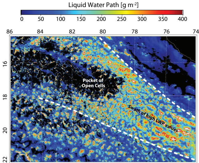
Fig. 09. MODIS-estimated cloud liquid water path (LWP) for the same overpass (1550 UTC) as shown in Fig. 01.
