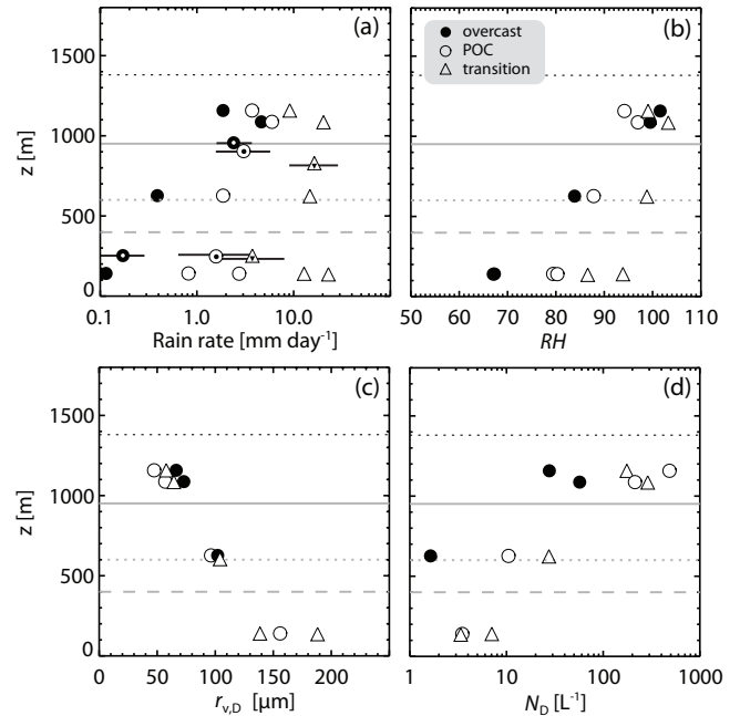
Fig. 08. Profiles of mean values of (a) precipitation rate (radar estimated values are shown for the height of maximum reflectivity and at 250 m by symbols with dots and horizontal bars show leg-leg variability), (b) relative humidity, (c) volume radius of drizzle drops, and (d) drizzle drop concentration in samples where the drizzle concentration exceeds 1 \text{ L}^{-1} . Symbolia are the same as for Fig. 06.
