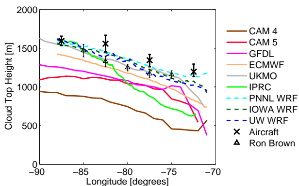
Figure 4. Model-mean cloud-top height along 20° S compared with mean cloud top measured using cloud radar from C-130 flights (Bretherton et al., 2010). Mean observations of R/V Ron Brown from 2001 to 2008 (de Szoeke et al., 2012) are plotted as triangles with bars as standard deviation.
