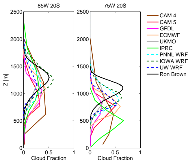
Figure 5. Mean model cloud fraction at 85° W, 20° S (left panel) and at 75° W, 20° S (right panel). Also plotted is cloud fraction inferred from R/V Ron Brown ship-based measurements over nearby longitudes from Burleyson et al. (2013). See text for more details.
