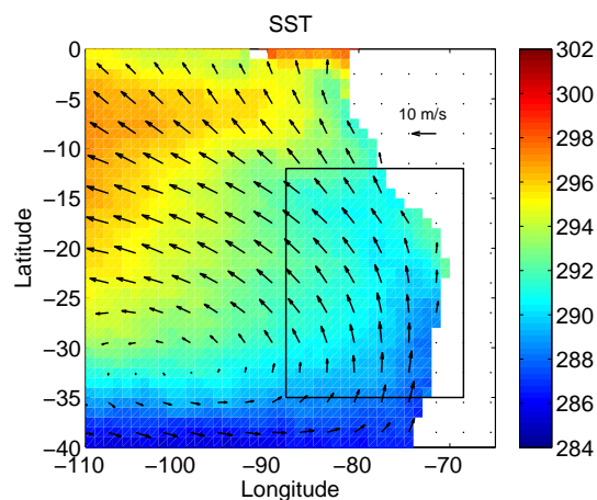
Figure 1. Observed SST (K) from AMSR-E and surface winds from QuikSCAT in the outer VOCA study region during the REx period, 15 October–16 November 2008. The inner study region is shown as a black rectangle.
