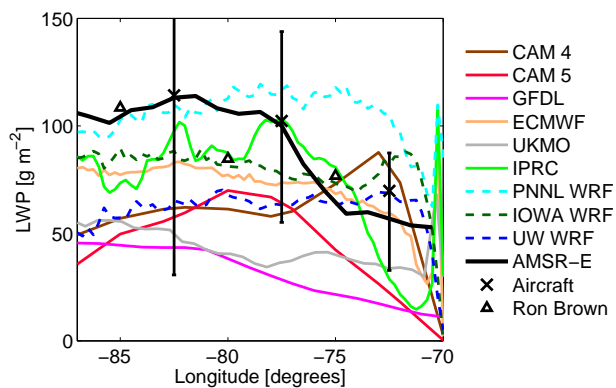
Figure 3. Grid-box mean LWP along 20° S compared with AMSR-E satellite mean of day and night passes and mean LWP from microwave radiometer on the C-130 (Zuidema et al., 2012). Error bars represent interquartile ranges of aircraft leg means. Also plotted as triangles are mean values measured by the R/V Ron Brown from 2001 to 2008 (de Szoeke et al., 2012).
