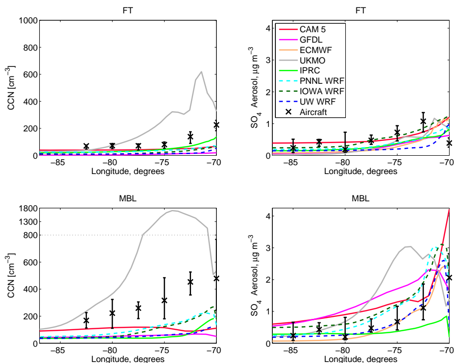
Figure 7. CCN concentrations at 0.1% supersaturation (in \text{cm}^{-3} ) along 20^\circ S are shown in the left-hand side panels. FT mean (top left) and concentration at 150 m (lower left). C-130 nephelometer means are plotted with “x” symbols. Sulfate aerosol ( \text{SO}_4 ) dry mass concentrations (in \mu\text{g m}^{-3} ) of diameter range 0.05\text{--}0.5\ \mu\text{m} measured with AMS (C-130 and BAE-146) are compared with model dry mass concentration along 20^\circ S (see Allen et al., 2011) in the right-hand side panels for the FT (top right) and MBL mean (bottom right). The lower-left panel is linearly rescaled at the top of the plot. The lower-right panel is modified from a figure in Mechoso et al. (2014) to add aircraft sampling variability. Note that ECMWF CCN concentrations are unavailable.
