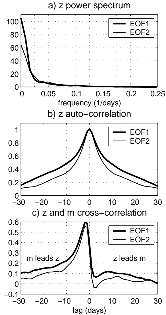
Figure 5 (a) Power spectrum for PC1 and PC2 of the vertical- and zonal- mean zonal wind. (b) Auto-correlation for PC1 and PC2 of the vertical- and zonal- mean zonal wind. The x-axis is time lag in days. (c) Cross-correlation between PC1 and its eddy forcing (thick line) and PC2 and its eddy forcing (thin line). Positive time lag means PC1 (zonal wind) leads the eddies ( m ).
