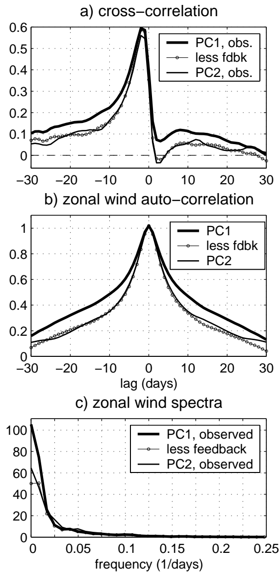
Figure 7 The effect of the stronger eddy-zonal wind feedback on the PC1 variability calculated from the simple model. (a) Same as Fig 5c. except that the calculated curve with the PC1 feedback reduced is also included (line with dots). (b) Same as Fig. 5b except that the calculated curve with the PC1 feedback reduced is also included (line with dots). (c) Same as Fig. 5a except that the calculated curve with the PC1 feedback reduced is also included (line with dots).
