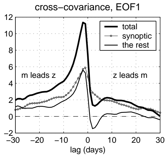
Figure 6 Cross-covariance between PC1 of the zonal wind and various components of the eddy forcing. The thick line is for the total eddy forcing, the line with dots is for the synoptic eddy forcing and the thin line is for the total eddy forcing minus the synoptic eddy forcing. Positive time lag means the zonal wind leads the eddies.
