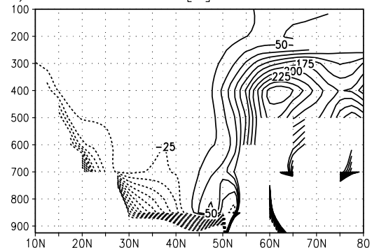
Figure 15 The difference in the quasi-geostrophic refractive index by stationary wave 1 (Low minus high index). The values are nondimensionalized by the radius of the earth squared. The differences are based on composites using the annular mode. (a) observed difference. (b) Contribution to the observed difference by the [u]_z terms. (c) Contribution to the observed difference by the [u]_{zz} term. (d) Contribution to the observed difference by both [u]_{zz} and the [u] in the denominator.
