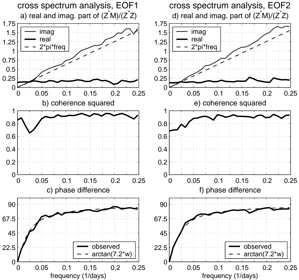
Figure 4 Cross spectrum analysis between the PC of the zonal wind and its eddy forcing. (a) The cross spectrum of PC1 and its eddy forcing divided by the PC1 power spectrum. Both the real and imaginary parts are shown as well as 2\pi times the frequency (dotted line). (b) Coherence squared function for PC1 and its eddy forcing. (c) Phase difference (in degrees) between PC1 of the zonal wind and its eddy forcing (solid line) and an estimate of the phase difference using (2) with \tau = 7.2 days (dotted line). Positive phase difference means the eddy forcing leads the zonal wind. (d), (e), and (f) are the same as (a), (b), and (c) except for PC2 instead of PC1.
