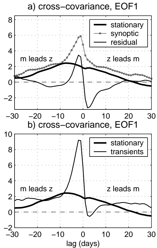
Figure 8 Cross-covariance between PC1 of the zonal wind and various components of the eddy forcing of PC1. Positive time lag means the zonal wind leads the eddies. (a) The thick line is for the quasi-stationary eddy forcing (including mountain torque), the line with dots is for the synoptic eddy forcing, and the thin line is for the residual eddy forcing (i.e. everything else).(b) The thick line is for the quasi-stationary eddy forcing (including mountain torque), the thin line is for the transient eddies (i.e. total minus quasi-stationary).
