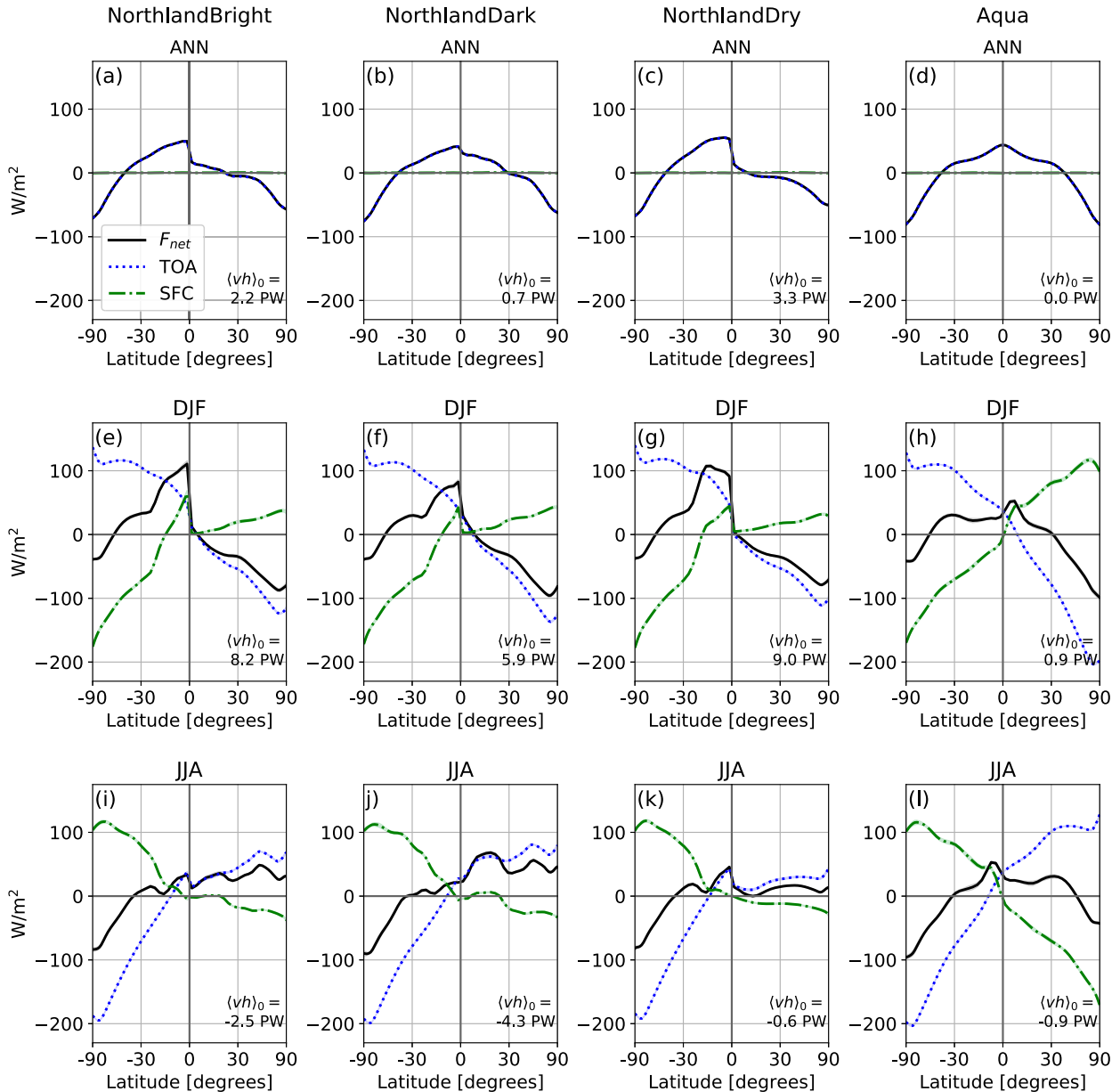
FIG. 12. Zonally averaged net TOA energy flux (TOA; blue dotted line), net surface energy flux (SFC; green dash-dotted line), and the atmospheric column energy source ( F_{net} = TOA - SFC ; black solid line) for the (top) annual mean, (middle) DJF, and (bottom) JJA. Shown are (a),(e),(i) NorthlandBright, (b),(f),(j) NorthlandDark, (c),(g),(k) NorthlandDry, and (d),(h),(l) Aqua. The total column-integrated cross-equatorial atmospheric energy transport (positive northward) for each season is noted in the lower right of each panel.
