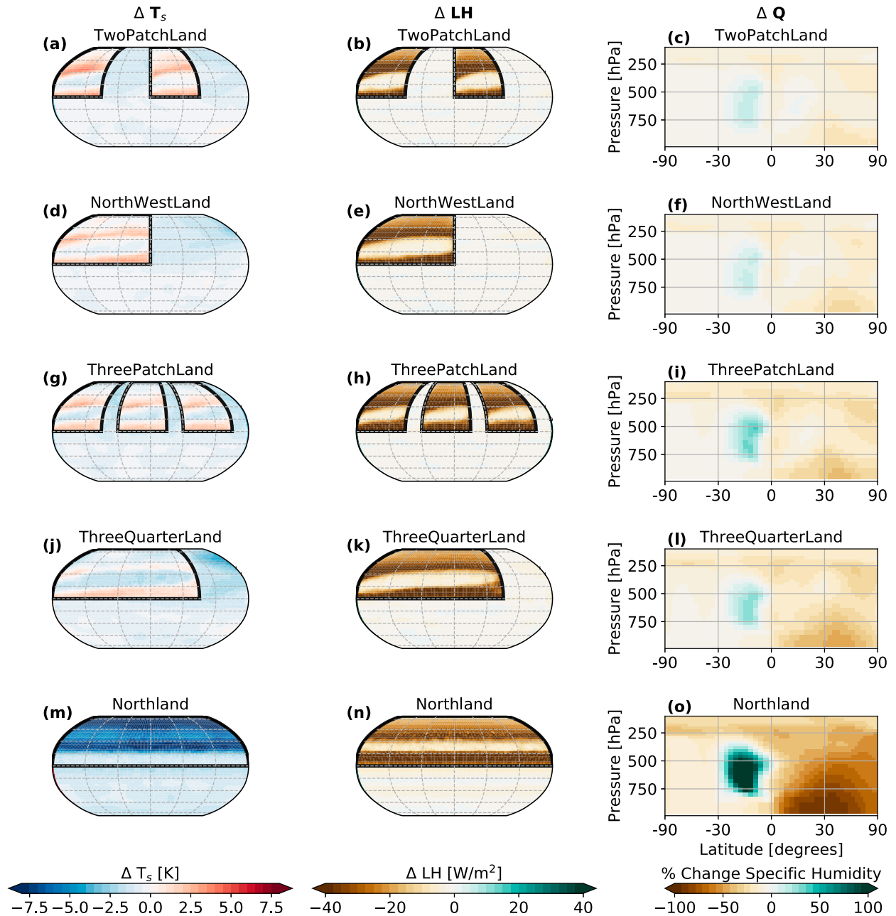
FIG. 7. Annual mean change in (left) surface temperature and (center) latent heat flux, and (right) percent change in zonal mean specific humidity for suppressing terrestrial evaporation in various continental configurations. Thick black lines show the continental boundary.
