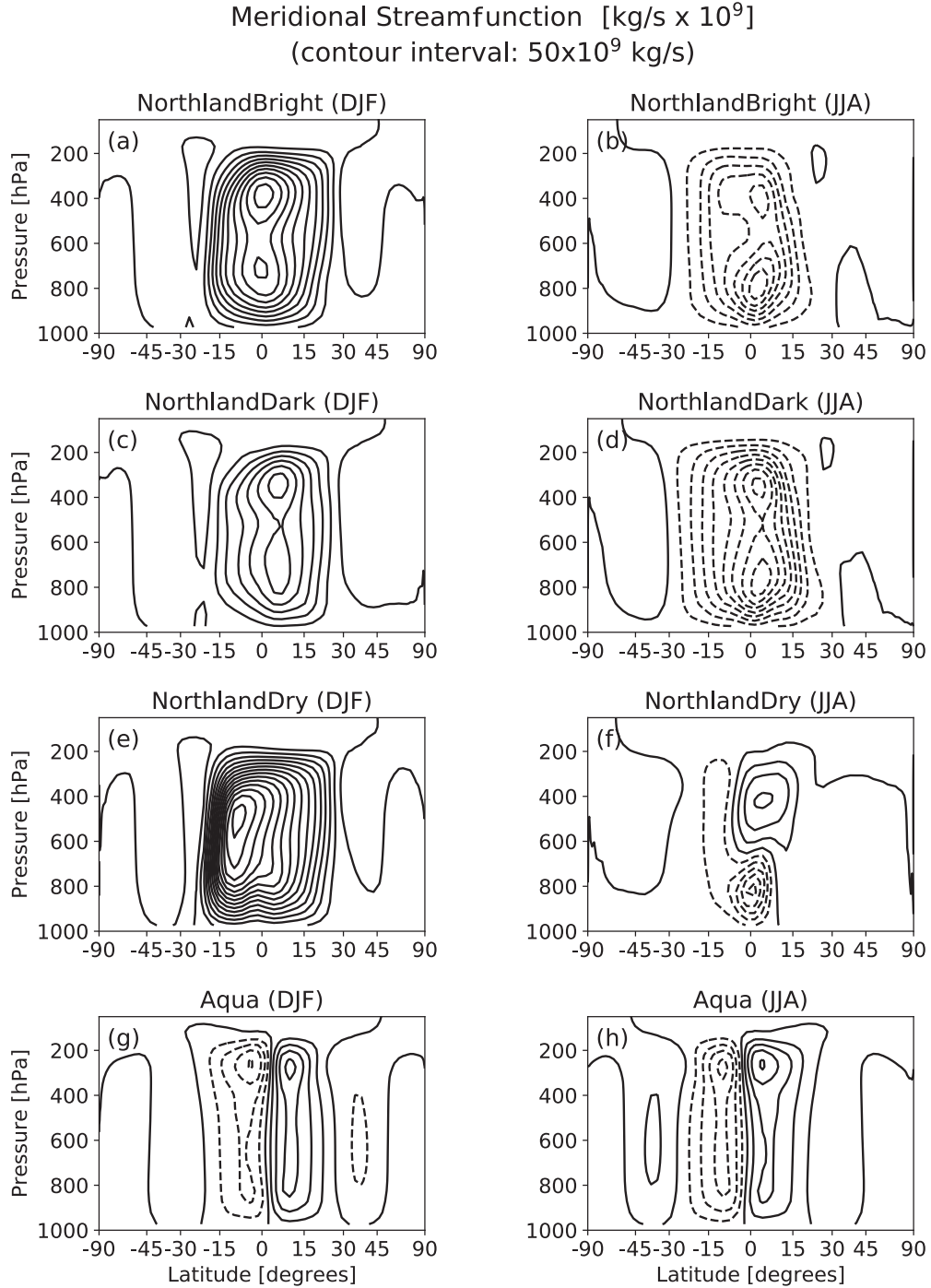
FIG. S3. Meridional streamfunction for DJF (left) and JJA (right) for NorthlandBright (a,b), NorthlandDark (c,d), NorthlandDry (e,f), and Aqua (g,h). Contours are spaced at 50 \times 10^9 \text{ kg/s} .
