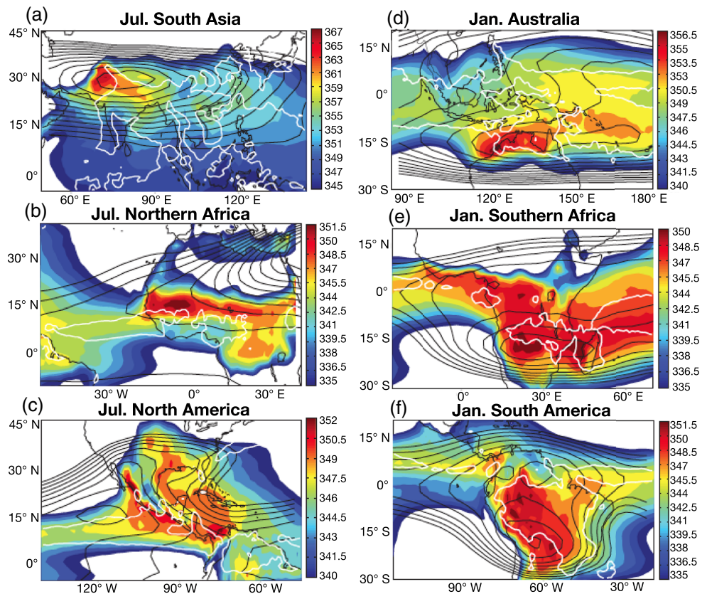
Figure 13. Evaluation of CQE for the (a) South Asia, (b) Northern Africa, (c) North America, (d) Australia, (e) Southern Africa, and (f) South America monsoons. Colors show subcloud equivalent potential temperature, \theta_{eb} . The black contour is the free-troposphere saturation equivalent potential temperature, \theta_e^* , averaged from 200 to 400 hPa. The white contour indicates the region that has precipitation greater than 6 mm/day. The \theta_e^* contours start from (a) 345 K, (b) 340 K, (c) 340 K, and (d–f) 341 K, and the respective interval is (a) 1 K, (b) 1 K, and (c–f) 0.5 K. Adapted from Nie et al. (2010). ©American Meteorological Society. Used with permission.
