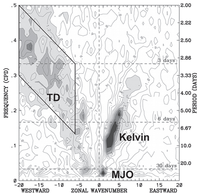
Figure 17. Wavenumber-frequency power spectrum of the symmetric component of OLR for June–August 1979–2003, averaged from 15°N to 15°S, plotted as the ratio of the raw OLR spectrum against a smooth red noise background (see Wheeler & Kiladis, 1999, for details). Contour interval is 0.1. Shading begins at 1.1, where the signal is statistically significant at approximately the 95% level. Peaks associated with the MJO, tropical depressions, and Kelvin waves are identified. From Kiladis et al. (2006). ©American Meteorological Society. Used with permission.
