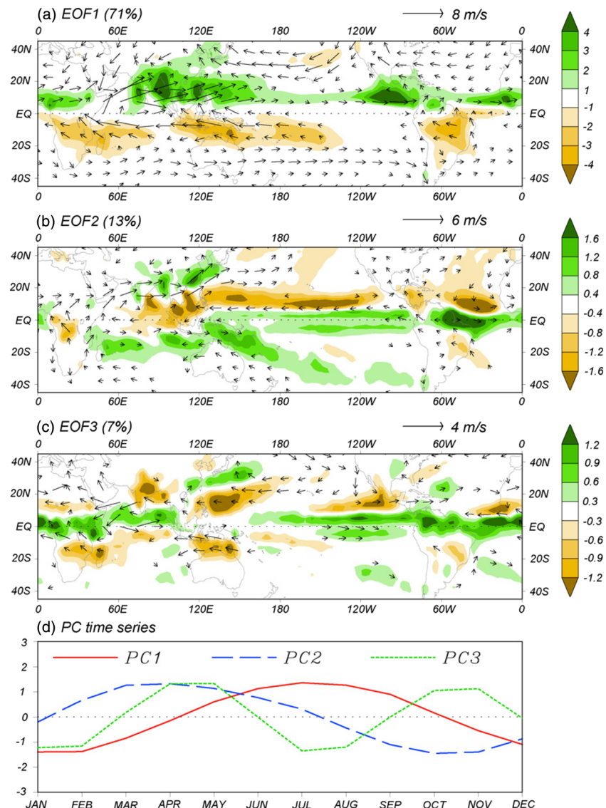
Figure 2. (a–c) The spatial patterns of the first three multivariable empirical orthogonal functions of the climatological monthly mean precipitation (colors, mm/day) and winds (arrows, m/s) at 850 hPa, and (d) their corresponding normalized principal components. Winds with speed less than 1 m/s are omitted. From Wang and Ding (2008). ©Elsevier. Used with permission.
