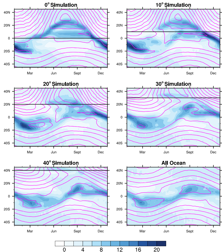
Figure 9. Seasonal cycles from idealized model simulations including simple continents with southern boundaries at 0°, 10°, 20°, 30°, and 40°, as well as an all-ocean aquaplanet. Land and ocean only differ in the corresponding mixed layer depth, which is 0.2 m for land and 20 m for ocean. Color contours show precipitation (contour interval 2 mm/day). Magenta contours indicate near-surface MSE taken at \sigma = 0.887 (contour interval 8 \times 10^3 \text{ J kg}^{-1} ). The southern boundary of land in each simulation is shown in a solid horizontal black line. Simulations were run using the Geophysical Fluid Dynamics Laboratory (GFDL) Flexible Modeling System (Frierson et al., 2006; O’Gorman & Schneider, 2008). Data can be accessed via CaltechDATA: (Bordoni, 2020).
