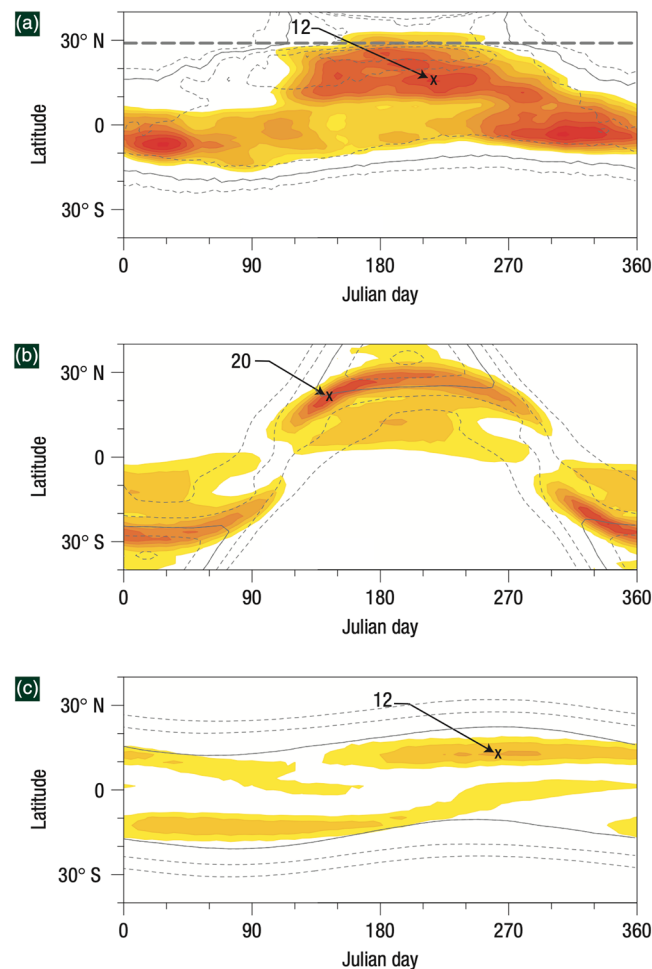
Figure 6. Seasonal cycle of zonal- and pentad-mean precipitation (color contours, data from GPCP 1999–2005) and sea level air temperature (gray contours, data from the ERA-40 reanalysis; Uppala et al., 2005) for (a) observations in the Asian monsoon sector (70–100°E), and for aquaplanet simulations with ocean mixed-layer heat capacity equivalent to (b) 0.5 m and (c) 50 m of water. The precipitation contour interval is 1 mm/day in (a) and 2 mm/day in (b) and (c), and maxima are indicated by crosses. For sea level air temperature, the contour interval is 2°C in all panels, and the solid gray line indicates the 24°C isotherm. The thick dashed line in (a) shows the latitude at which the zonal-mean topography in the Asian monsoon sector rises above 3 km. From Bordoní and Schneider (2008). Note that mixed layer depths here are corrected from Bordoní and Schneider (2008), (S. Bordoní, personal communication, 02/18/2020).
