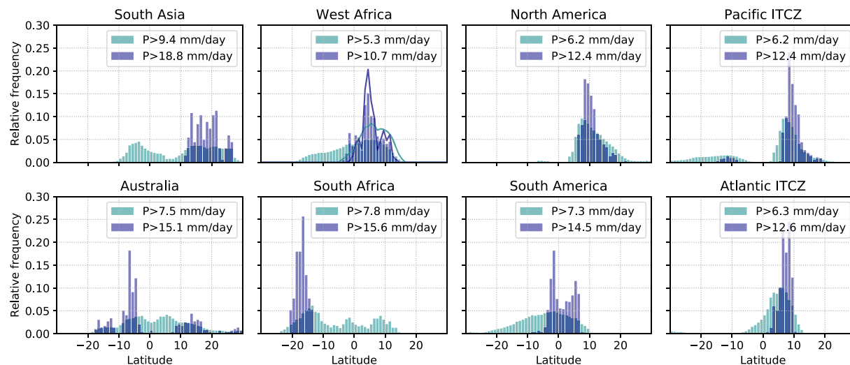
Figure 15. Relative frequency distributions of latitudes where the strongest precipitation falls in the regional monsoons and ITCZs. Monsoon regions are defined as in Figure 1, and ITCZs as in Figure 10. For West Africa, lines show the distribution for -10^{\circ}\text{E} to 10^{\circ}\text{E} . Data are from a linearly detrended pentad-mean climatology of GPCP precipitation data spanning 1997–2014.
