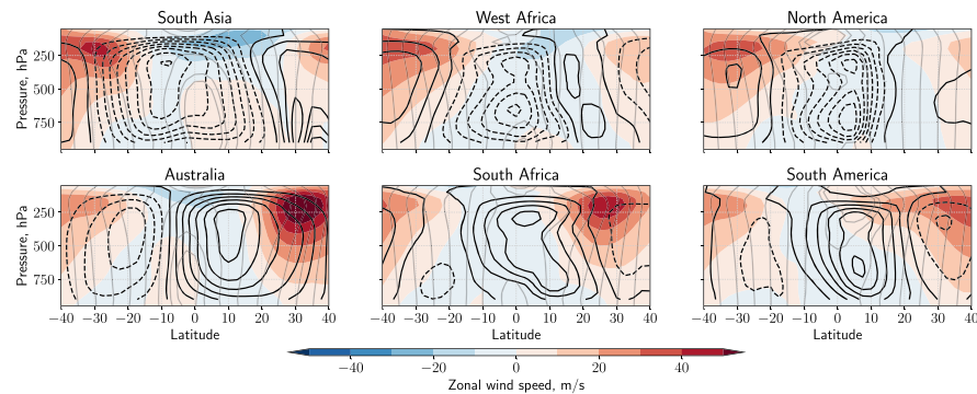
Figure 14. Black contours show local summer (June–September or December–March) meridional overturning circulations for South Asia (70–100°E), West Africa (10°W to 30°E), North America (85–115°W), Australia (115–155°E), South Africa (10–50°E), and South America (40–70°W). This is computed by vertically integrating the divergent component of the meridional wind, averaged in longitude, from the top of the atmosphere to the surface (cf. Schwendike et al., 2014; Zhang & Wang, 2013). Shading shows zonal wind. Light gray contours indicate absolute angular momentum per unit mass, with contours at \Omega a^2 \cos^2 \phi_i ( \phi_i = 0^\circ, \pm 5^\circ \pm 10^\circ, \dots ).
