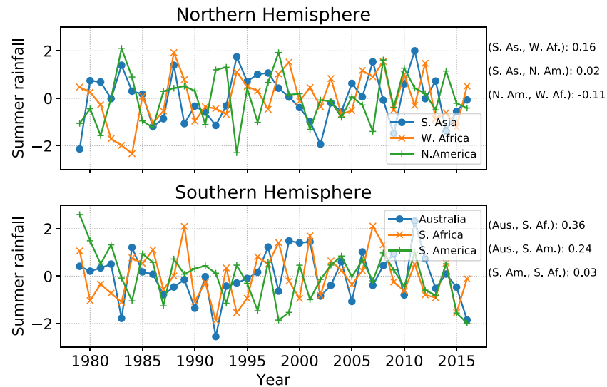
Figure 3. Time series of summertime (June–September mean in the Northern Hemisphere and December–March mean in the Southern Hemisphere) rainfall averaged over the yellow boxes marked in Figure 1, which are used as approximations to the monsoon regions defined by the magenta contour. For ease of comparison, the time series are standardized by subtracting the mean and dividing by the standard deviation. Pearson correlation coefficients are given to the right of the figure; except for the correlation between Australian and Southern African rainfall, correlations are not significantly different from 0 ( p = 0.10 ). Data are taken from the Global Precipitation Climatology Project (GPCP Huffman et al., 2001) over 1979–2016.
