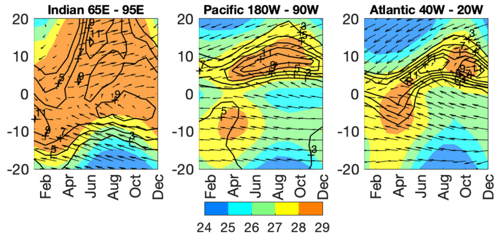
Figure 10. Hovmöller diagram of the climatological SST and 10 m wind averaged across the (left) Indian, (center) eastern half of the Pacific, and (right) Atlantic basin. SST is shaded (in °C), and precipitation is contoured (contour interval 2 mm/day). The wind vectors are relative to the maximum in each panel. Precipitation data are from CMAP 1979–2017 (Xie & Arkin, 1997), SST data are from HADISST 1870–2017 (Rayner et al., 2003), and wind data are from ERA-Interim 1979–2017 (Dee et al., 2011). From Battisti et al. (2019). ©American Meteorological Society. Used with permission.
