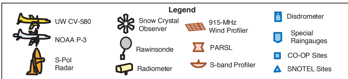
Figure 1.1. Observing facilities for IMPROVE-II.
