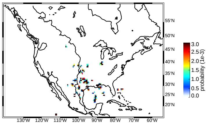
(e) MAM wide convective cores strong thresholds
