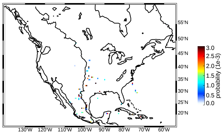
(c) MAM deep/wide convective cores strong thresholds
