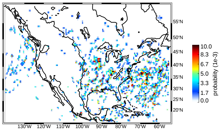
(e) MAM wide convective cores moderate thresholds
