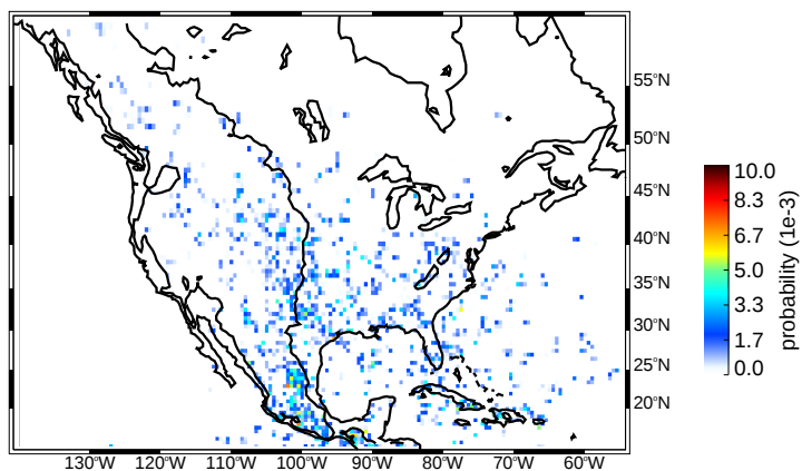
(c) MAM deep/wide convective cores moderate thresholds
