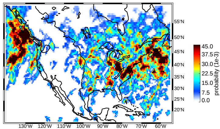
(f) MAM broad strat regions between mod & str thresholds
