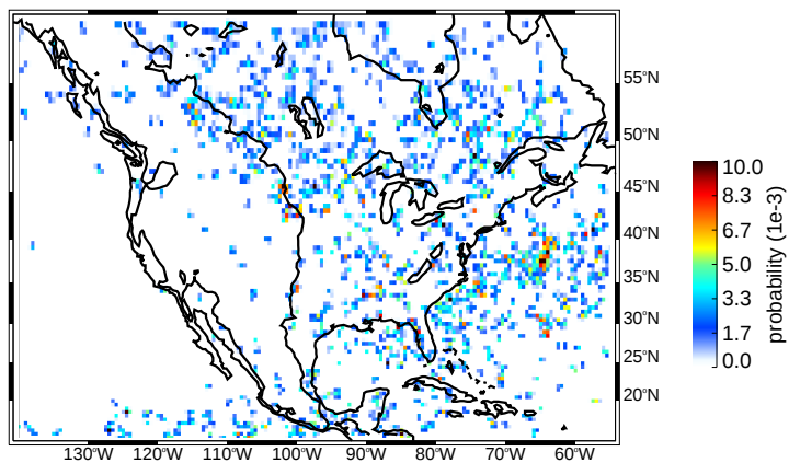
(e) JJA wide convective cores moderate thresholds
