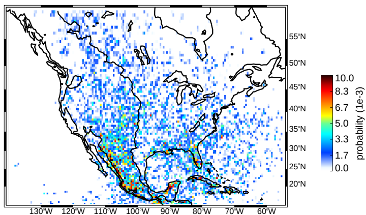
(c) JJA deep/wide convective cores moderate thresholds
