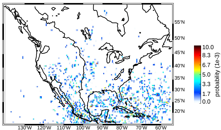
(c) SON deep/wide convective cores moderate thresholds
