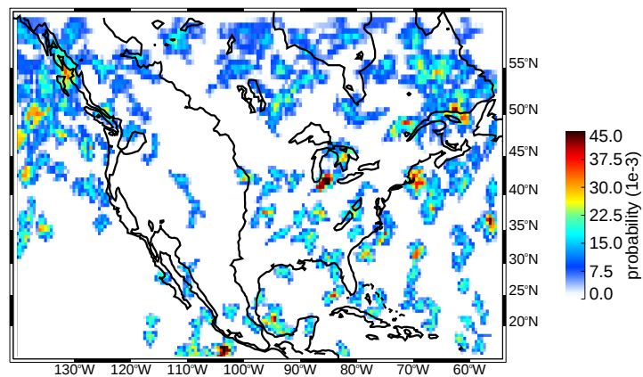
(f) SON broad strat regions between mod & str thresholds
