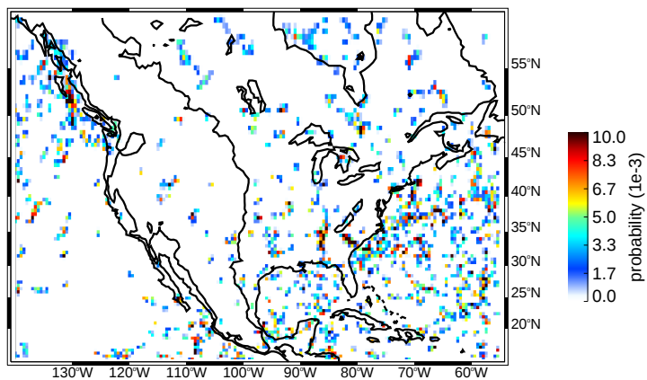
(e) SON wide convective cores moderate thresholds
