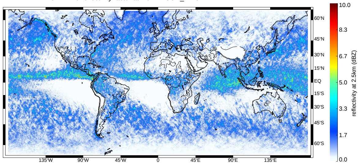
GPM 2Ku reflectivity factor at 2.5km - SON_1415
