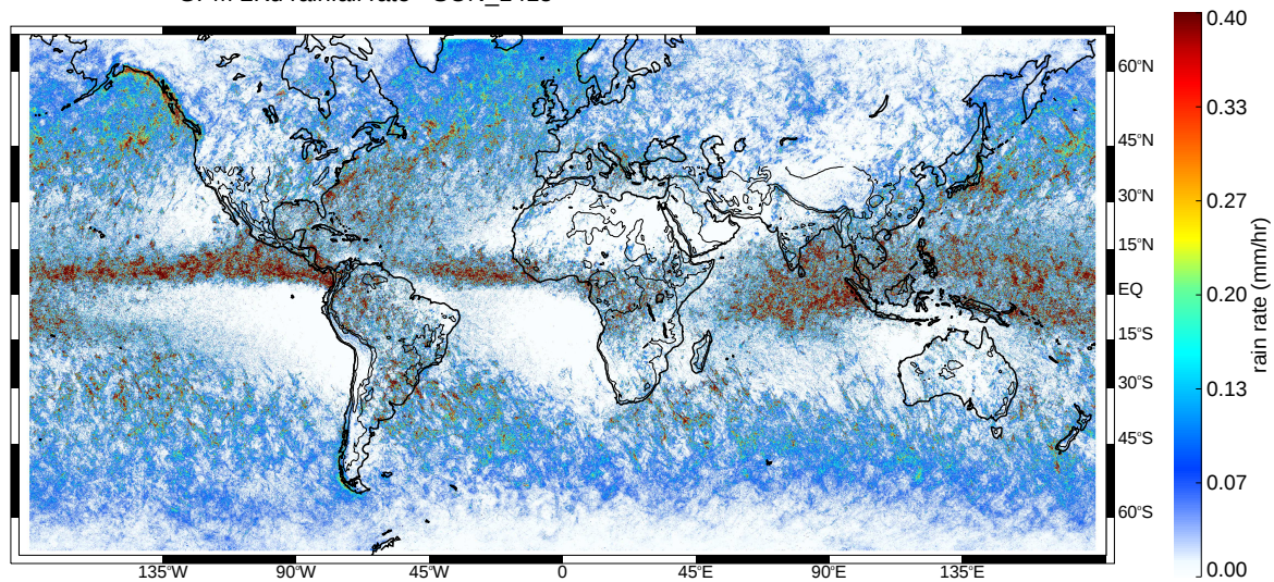
GPM 2Ku rainfall rate - SON_1415
