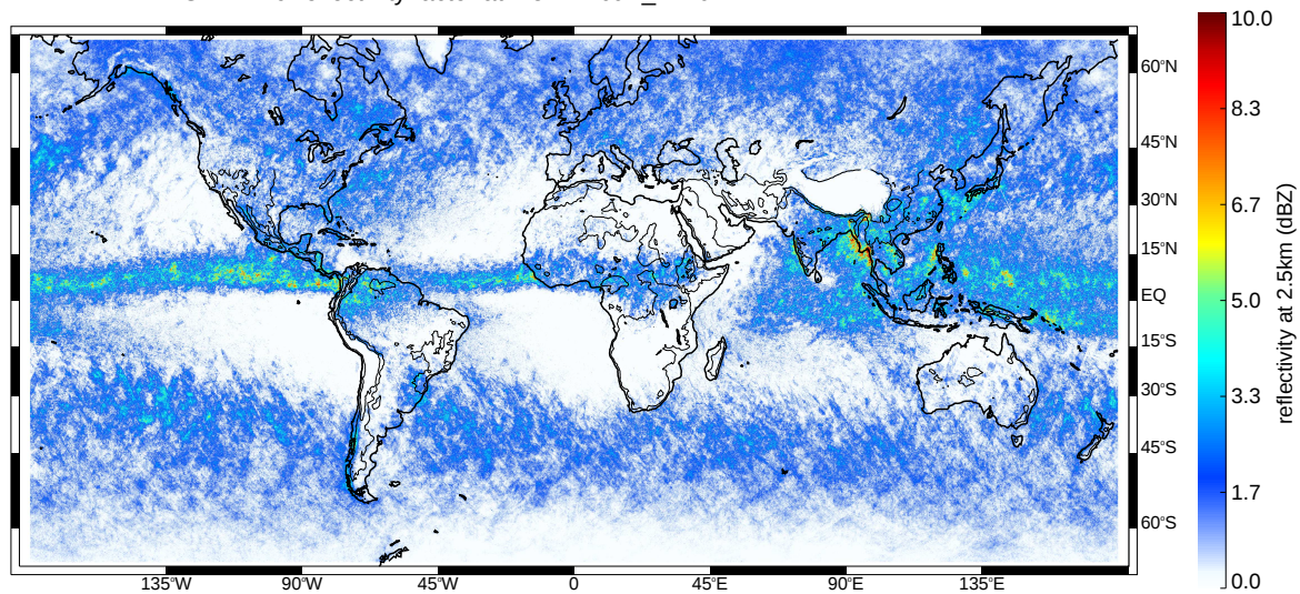
GPM 2Ku reflectivity factor at 2.5km - JJA_1416
