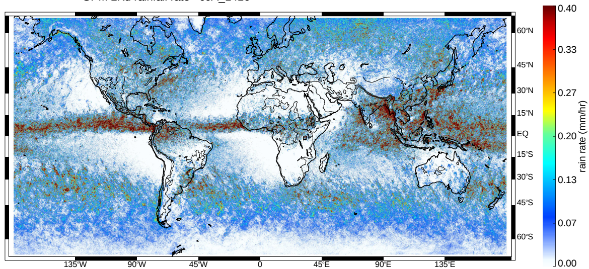
GPM 2Ku rainfall rate - JJA_1416
