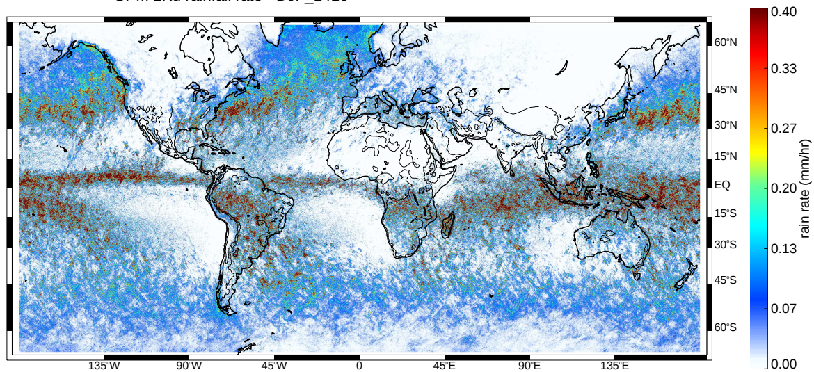
GPM 2Ku rainfall rate - DJF_1416
