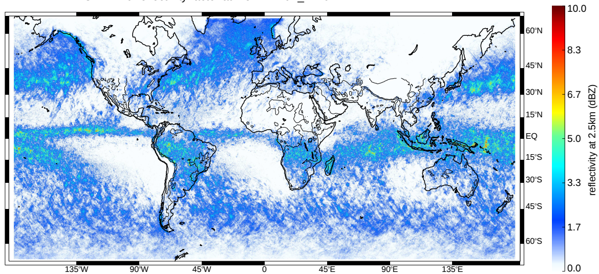
GPM 2Ku reflectivity factor at 2.5km - DJF_1416
