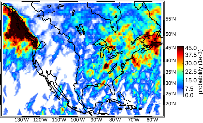
(a) SON broad stratiform regions
