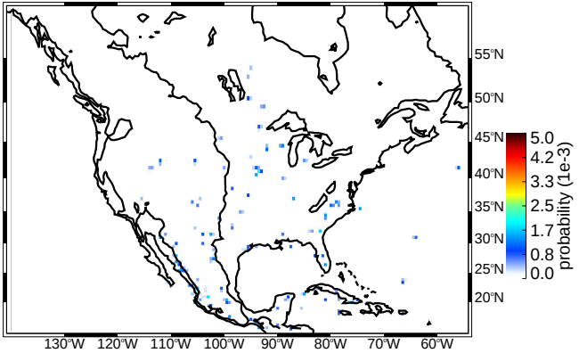
(b) SON deep convective cores
