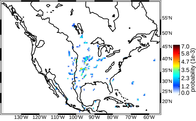
(c) SON deep/wide convective cores
