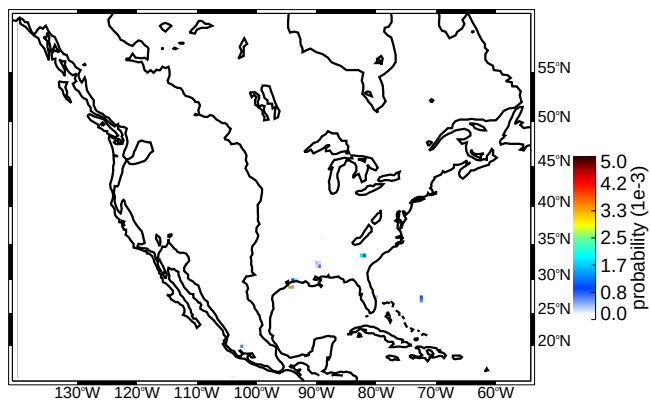
(b) DJF deep convective cores
