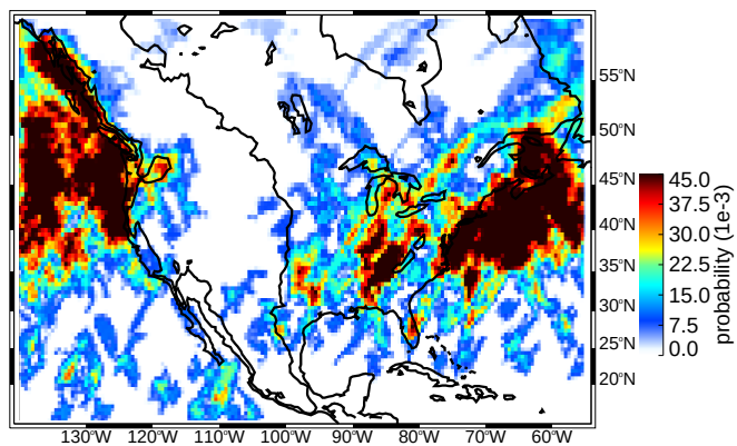
(a) DJF broad stratiform regions
