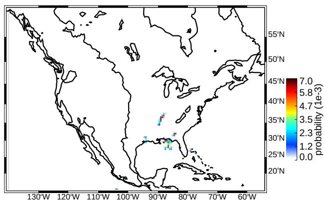
(c) DJF deep/wide convective cores
