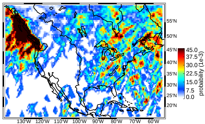
(a) SON broad stratiform regions
