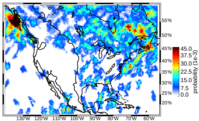
(a) JJA broad stratiform regions
