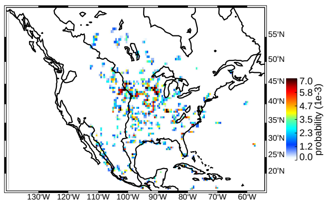
(c) JJA deep/wide convective cores
