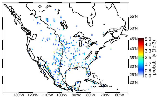
(b) JJA deep convective cores
