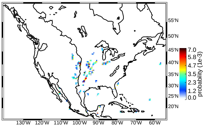
(c) SON deep/wide convective cores strong thresholds (uw)
