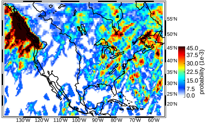
(a) SON broad stratiform regions strong thresholds (uw)
