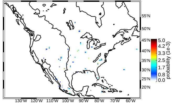
(b) SON deep convective cores strong thresholds (uw)
