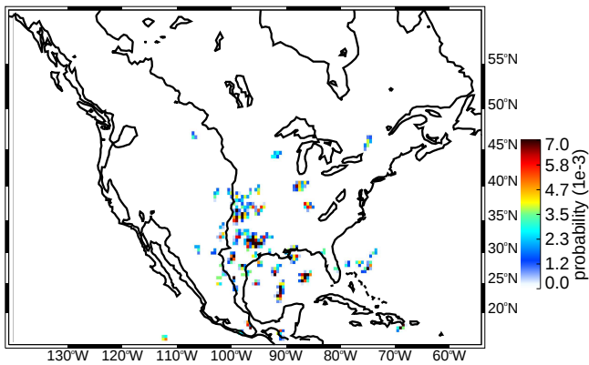
(c) MAM deep/wide convective cores strong thresholds (uw)
