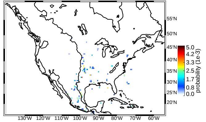
(b) MAM deep convective cores strong thresholds (uw)
