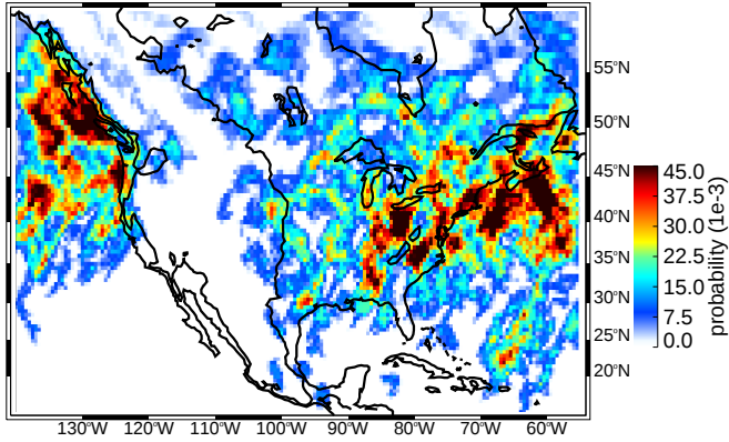
(a) MAM broad stratiform regions strong thresholds (uw)
