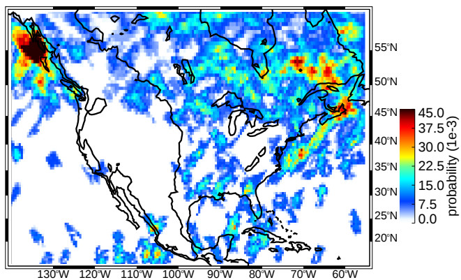
(a) JJA broad stratiform regions strong thresholds (uw)
