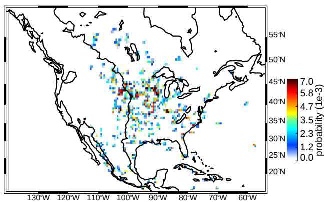
(c) JJA deep/wide convective cores strong thresholds (uw)
