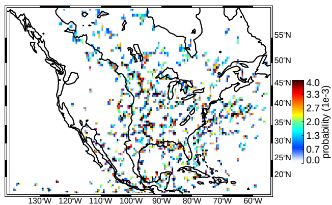
(d) JJA wide convective cores strong thresholds (uw)
