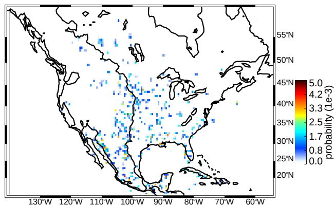
(b) JJA deep convective cores strong thresholds (uw)
