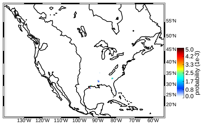
(b) DJF deep convective cores strong thresholds (uw)
