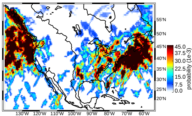
(a) DJF broad stratiform regions strong thresholds (uw)
