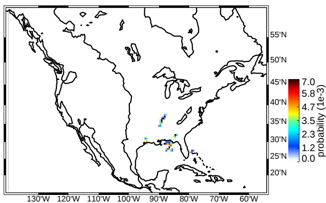
(c) DJF deep/wide convective cores strong thresholds (uw)
