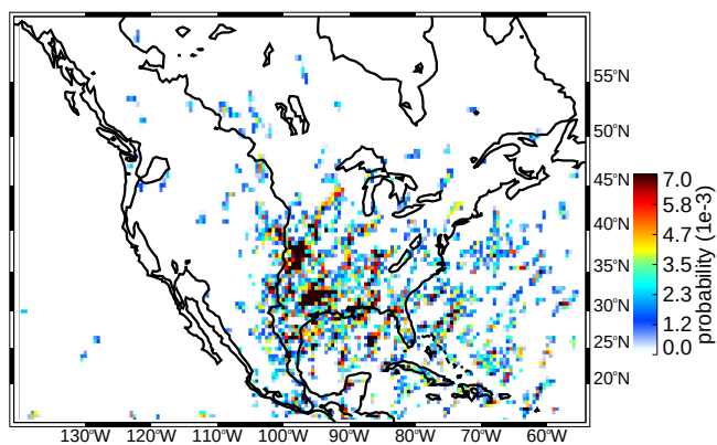
(c) MAM deep/wide convective cores
