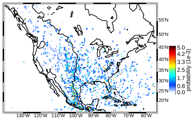
(b) MAM deep convective cores
