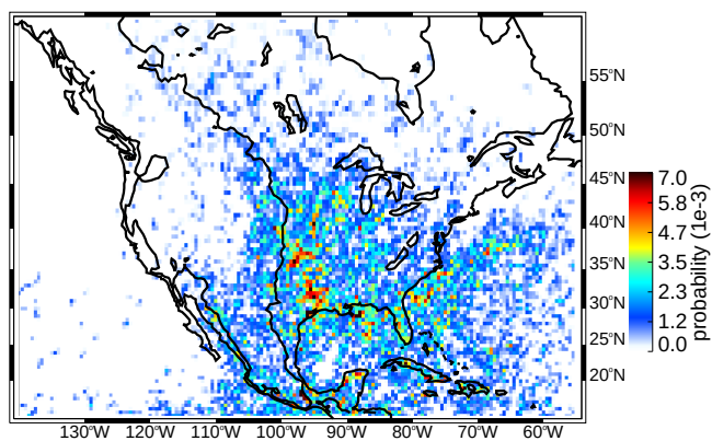
(c) J-D deep/wide convective cores
