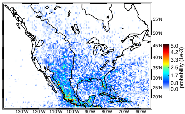
(b) J-D deep convective cores
