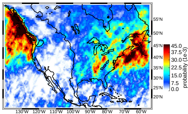
(a) J-D broad stratiform regions
