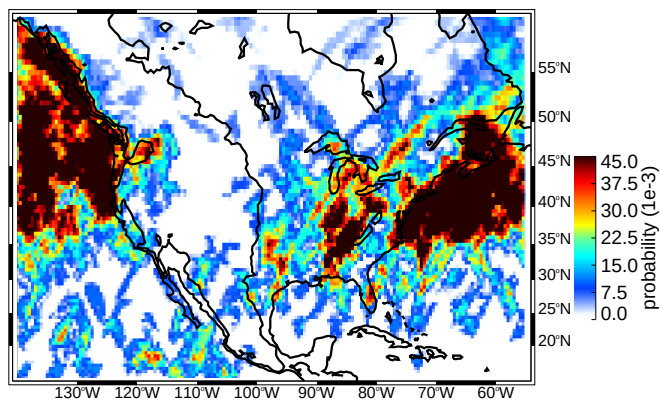
(a) DJF broad stratiform regions
