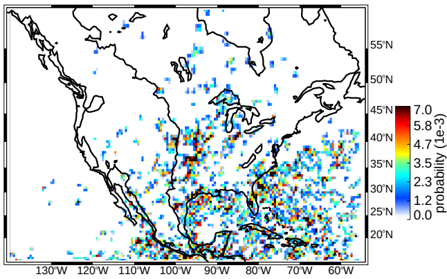
(c) SON deep/wide convective cores moderate thresholds (uw)
