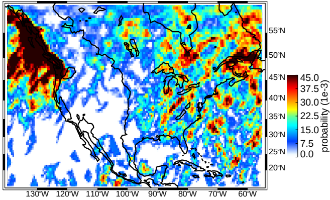
(a) SON broad stratiform regions moderate thresholds (uw)
