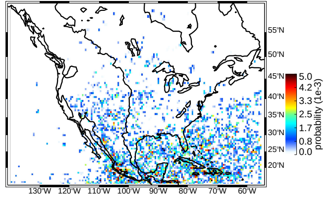
(b) SON deep convective cores moderate thresholds (uw)
