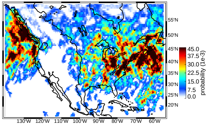
(a) MAM broad stratiform regions moderate thresholds (uw)
