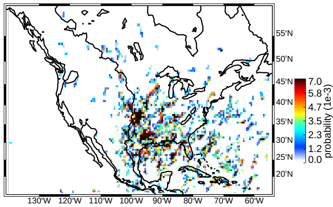
(c) MAM deep/wide convective cores moderate thresholds (uw)
