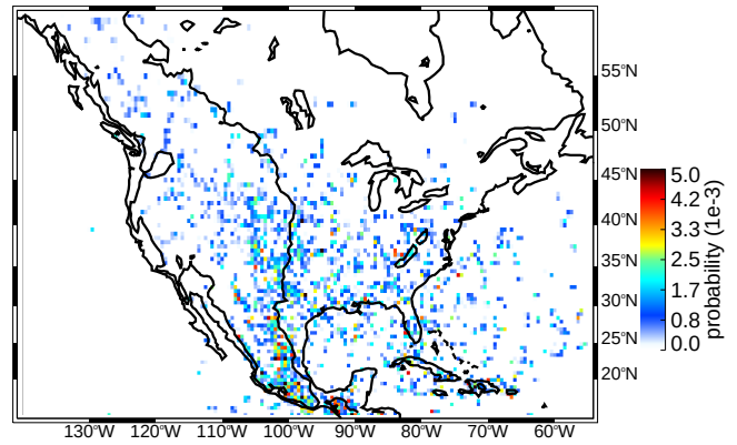
(b) MAM deep convective cores moderate thresholds (uw)
