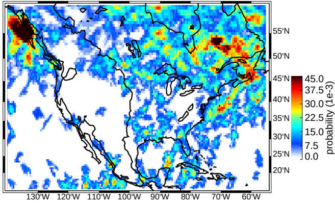
(a) JJA broad stratiform regions moderate thresholds (uw)
