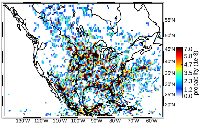
(c) JJA deep/wide convective cores moderate thresholds (uw)
