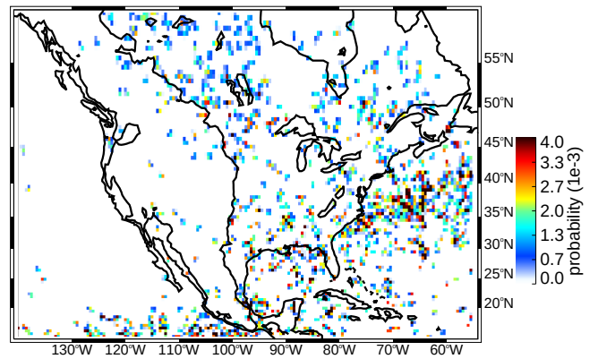
(d) JJA wide convective cores moderate thresholds (uw)
