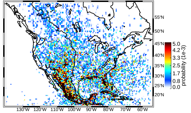
(b) JJA deep convective cores moderate thresholds (uw)
