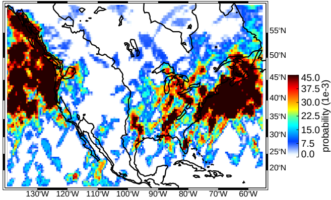
(a) DJF broad stratiform regions moderate thresholds (uw)
