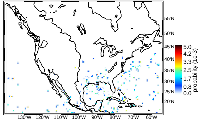
(b) DJF deep convective cores moderate thresholds (uw)
