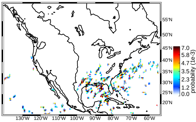
(c) DJF deep/wide convective cores moderate thresholds (uw)
