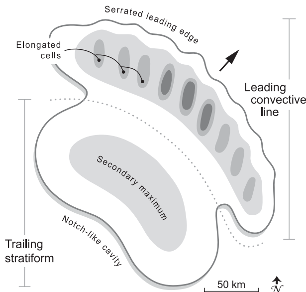
FIG. 14. Schematic of the leading-line/trailing-stratiform arch-type described in Houze et al. (1990), but reoriented for study in the Southern Hemisphere. Increasing levels of shading indicate more intense radar reflectivity. As described in section 6, storms with wide convective cores were systematically compared to this idealized structure.
