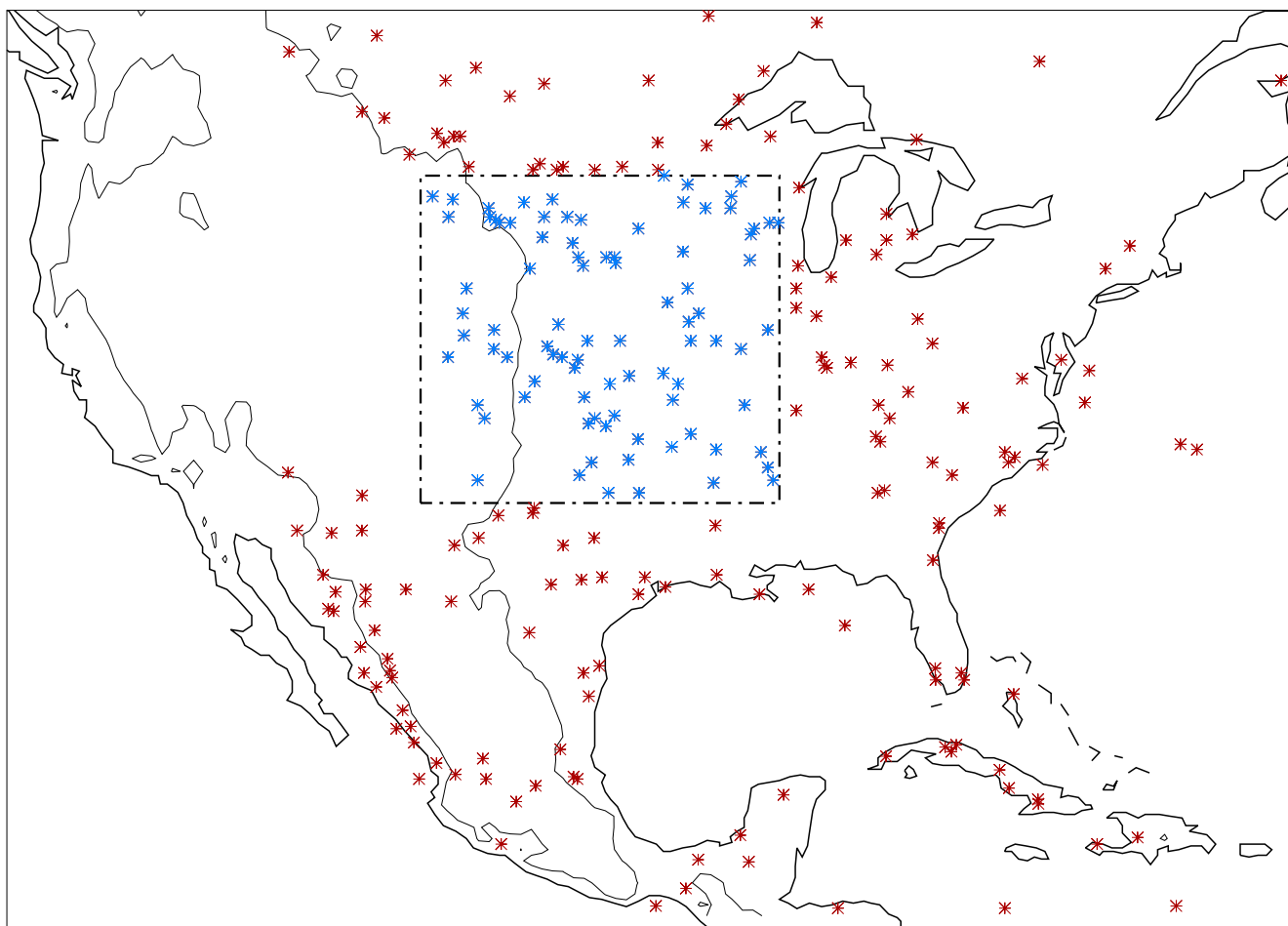
Location of DWCC event centroids for str_JJA n=261
