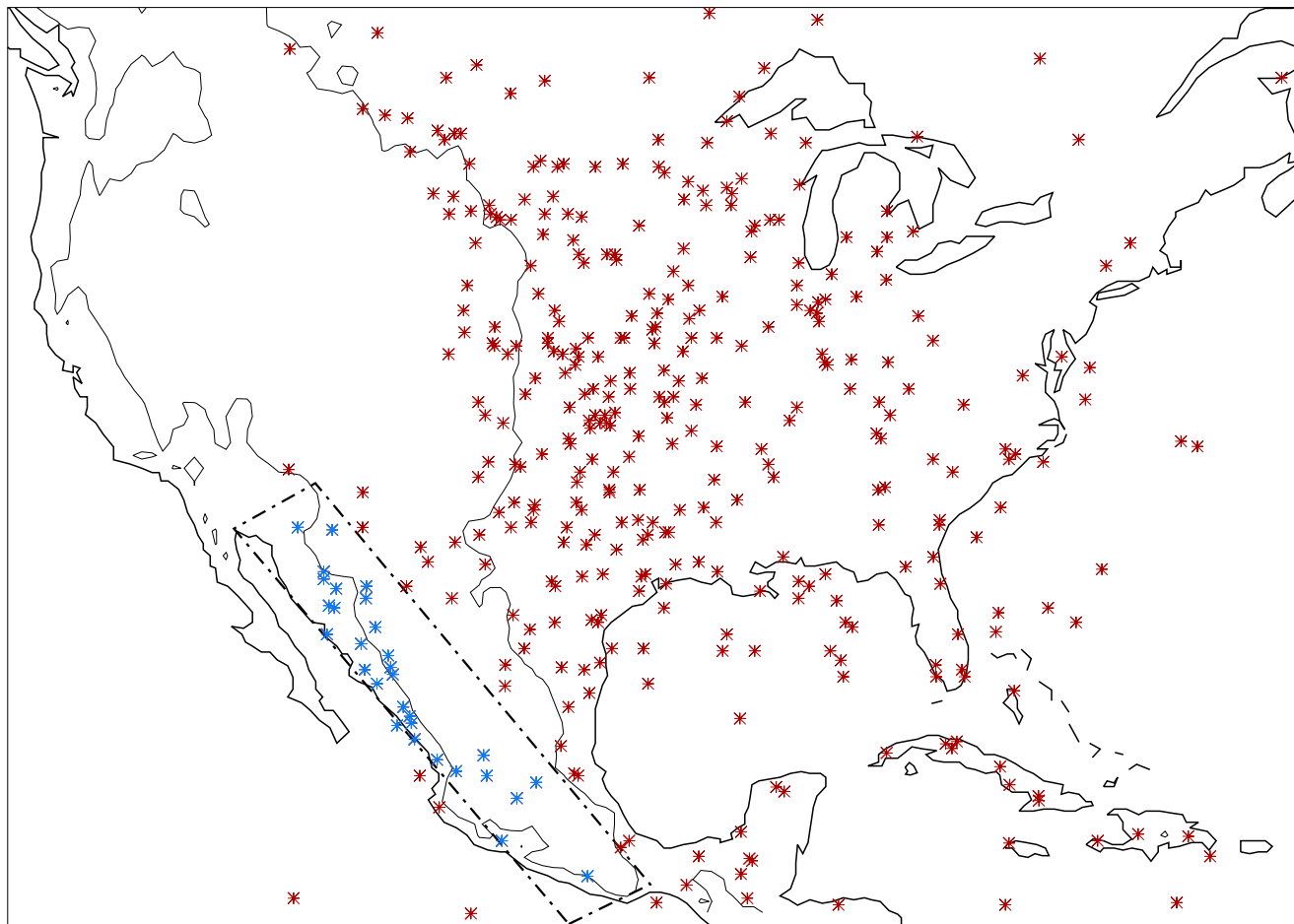
Location of DWC event centroids for Mar 2014 – Apr 2018, str thresholds total=397 & n=27
