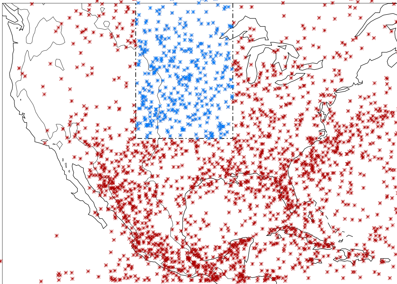
Location of DWCC event centroids for mod_JJA n=2783
