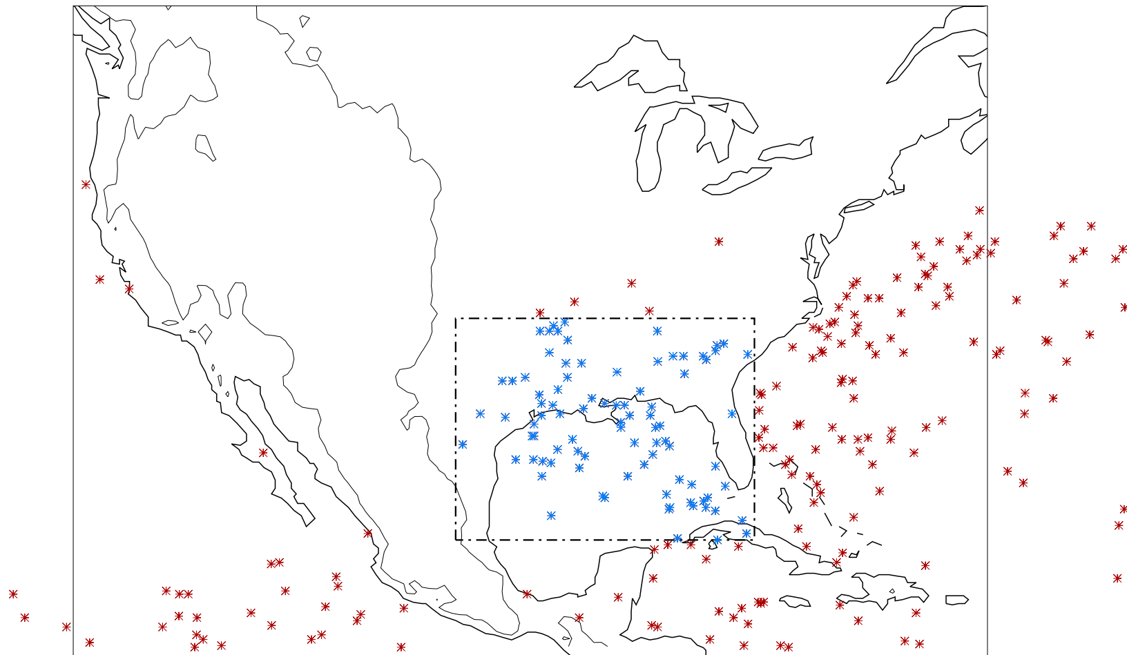
Location of DWCC event centroids for mod_DJF n=269
