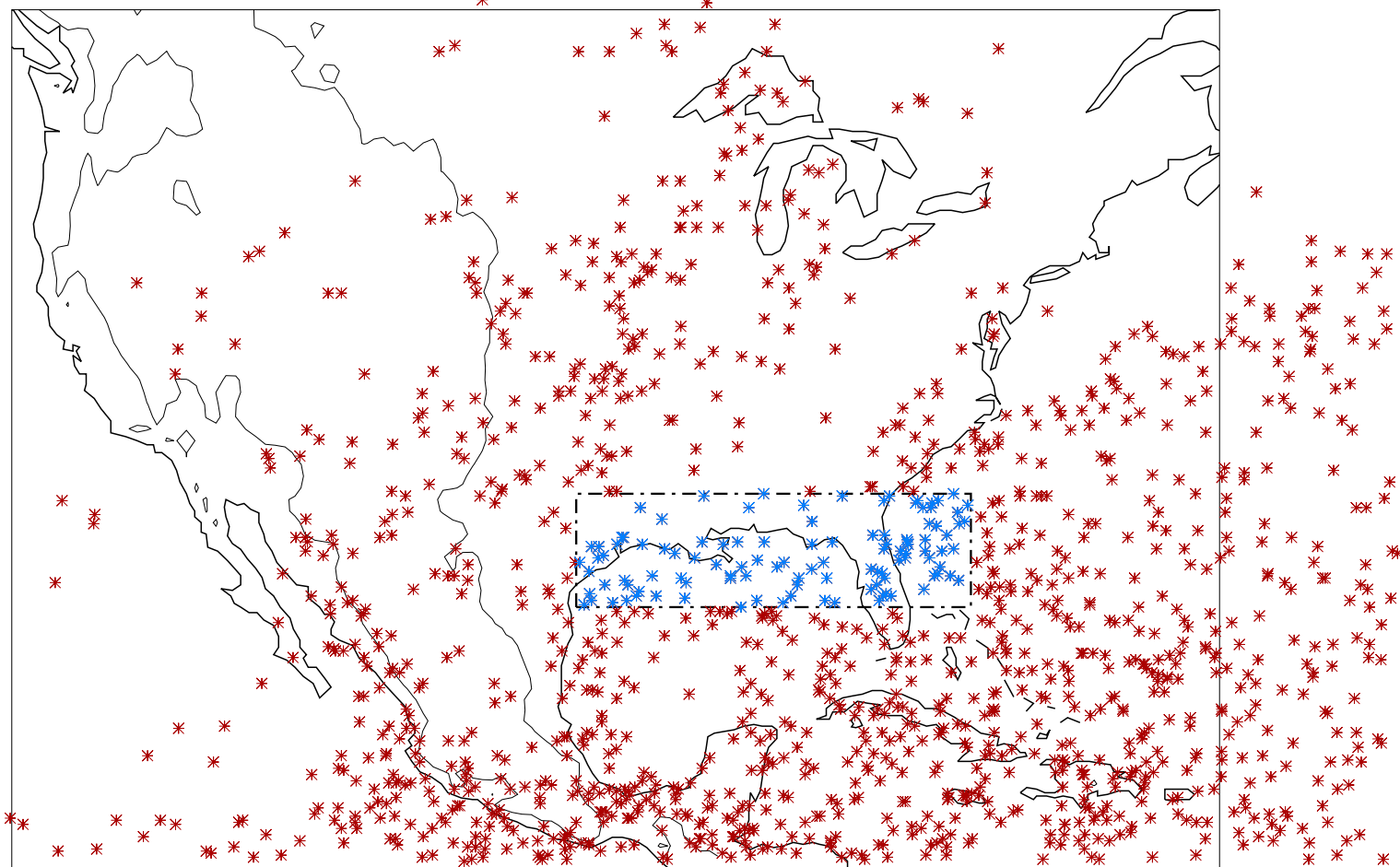
Location of DWCC event centroids for mod_SON n=1331
