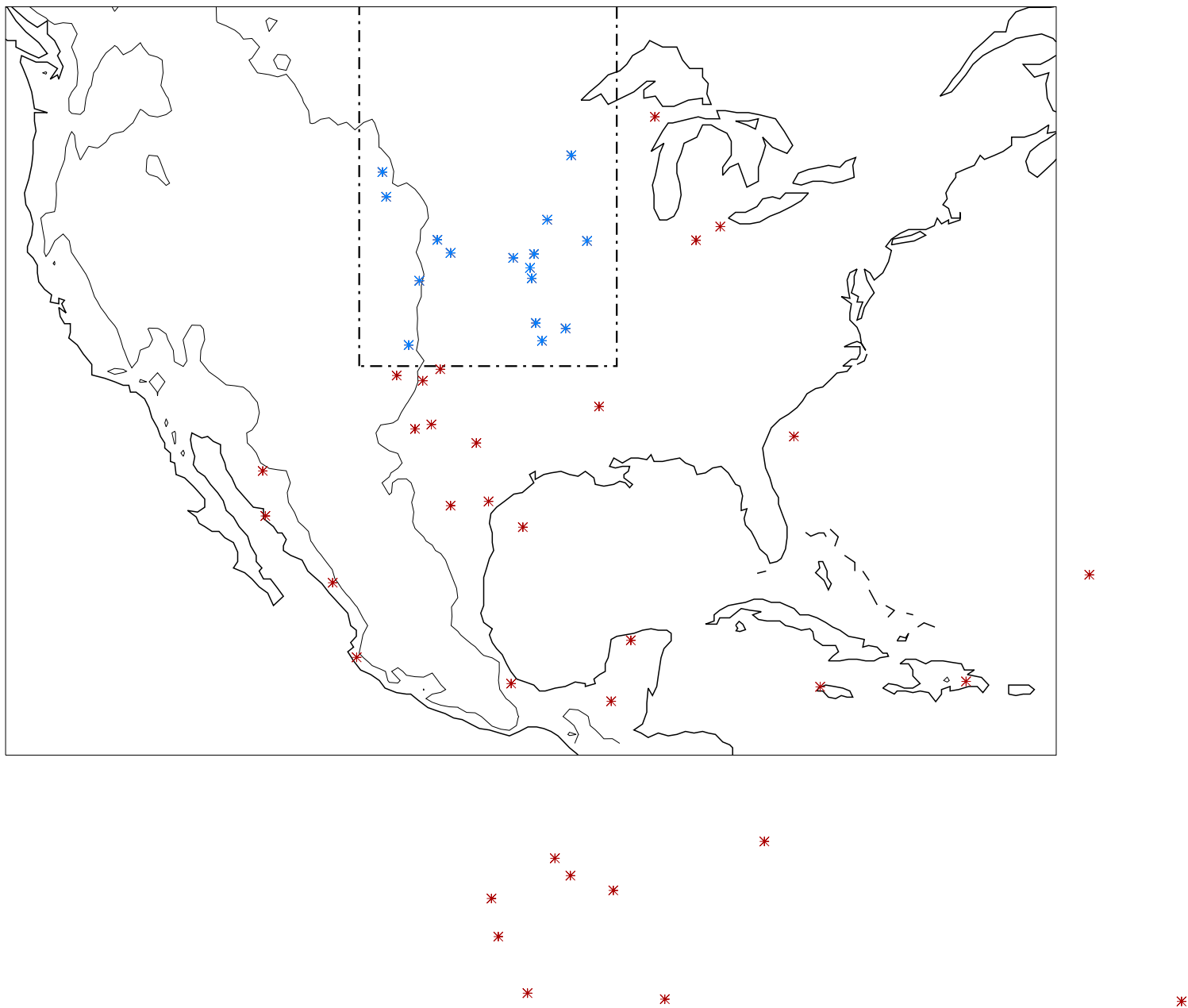
Location of DWCC event centroids for v9_SON n=49
