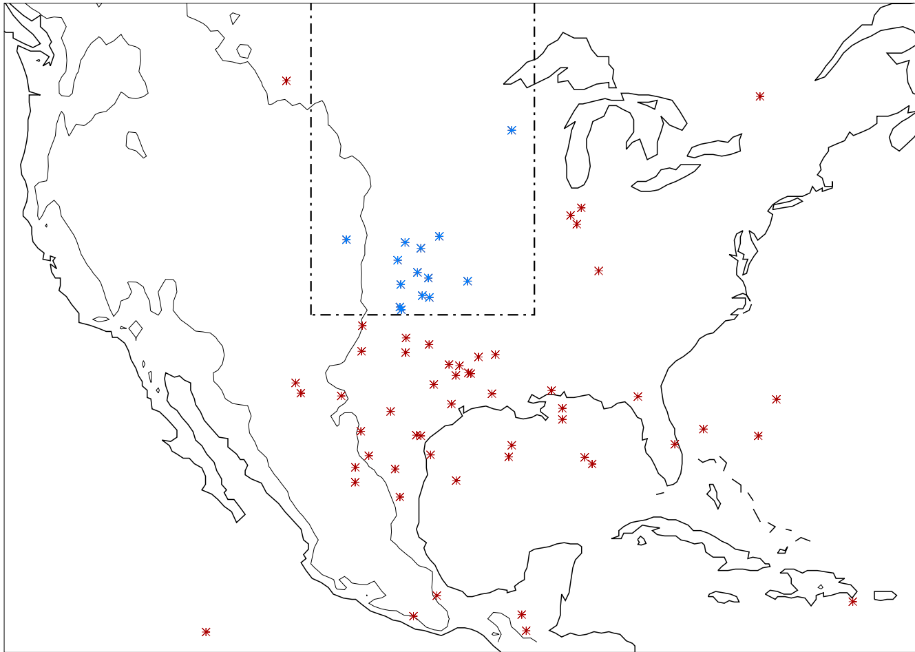
Location of DWCC event centroids for v9_MAM n=79
