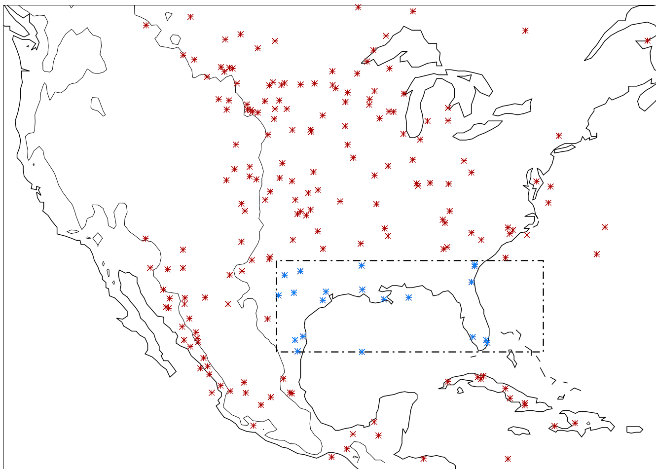
Location of DWCC event centroids for v9_JJA n=260
