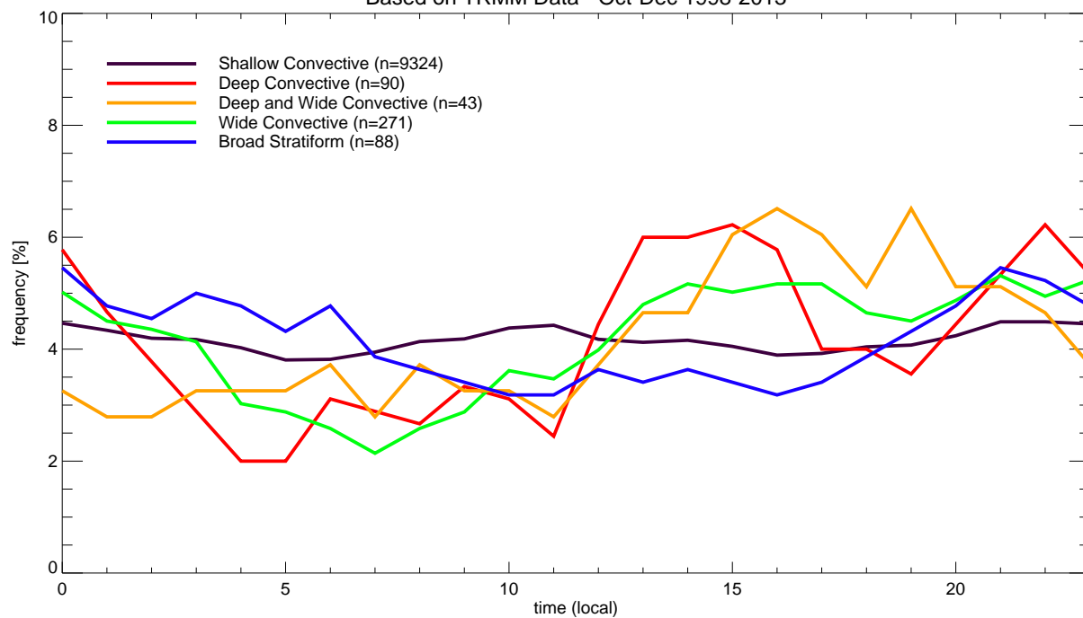
Based on TRMM Data - Oct-Dec 1998-2013
