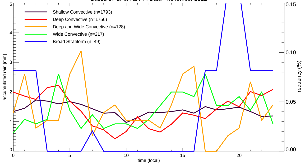
Based on SPol-Ka PPI Data - November 2011
