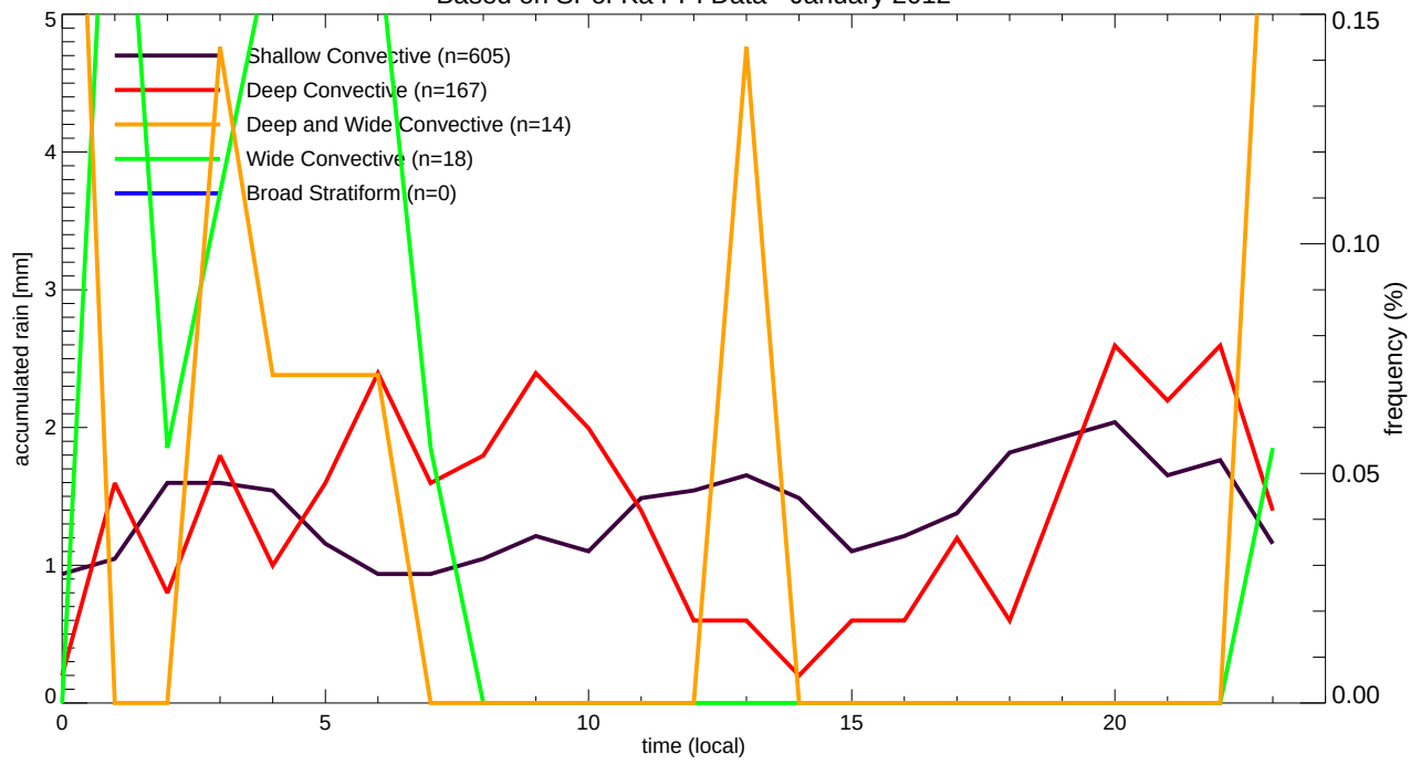
Based on SPol-Ka PPI Data - January 2012
