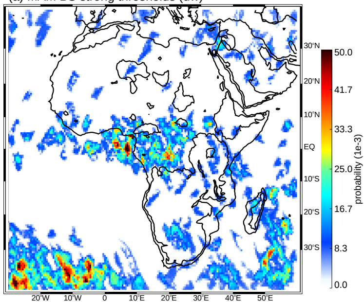
(a) MAM BS strong thresholds (uw)
