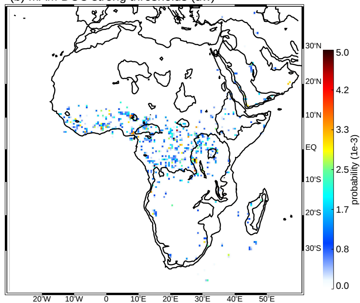
(b) MAM DCC strong thresholds (uw)
