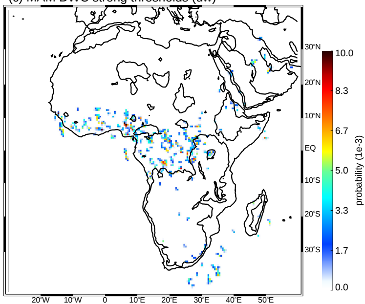
(c) MAM DWC strong thresholds (uw)
